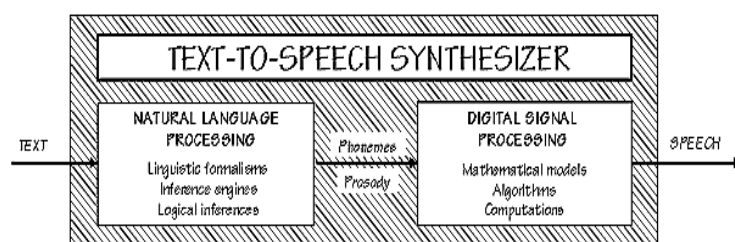
Figure 1: A simple but general functional diagram of a TTS system. [2]
