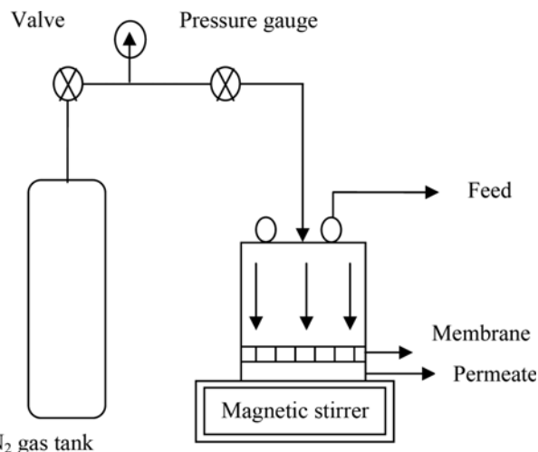
Fig. 1. Schematic diagram showing a dead end cell.
