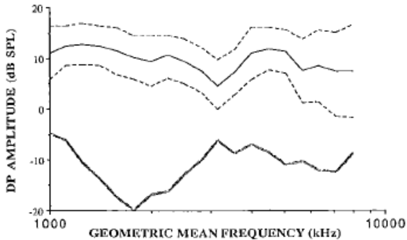
Figure 1. Distortion product emission (DPE) audio-gram. Mean DPE amplitude \pm 1 SD is presented as fine lines and noise floor plus 1 SD as solid line. They are plotted at geometric mean of primary tones to correspond to region of generation on basilar membrane; the intensity of stimulation is 75 dB SPL for L_1 = L_2
