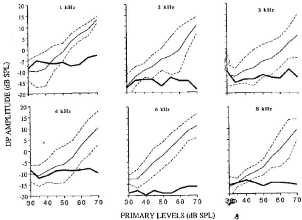
Figure 2. Distortion product emission (DPE) input-output functions obtained at six frequencies with equi-level primaries whose geometric means represent the frequency of study. Mean DPE amplitude \pm 1 SD is presented in fine lines and associated noise floors plus 1 SD as solid line.
