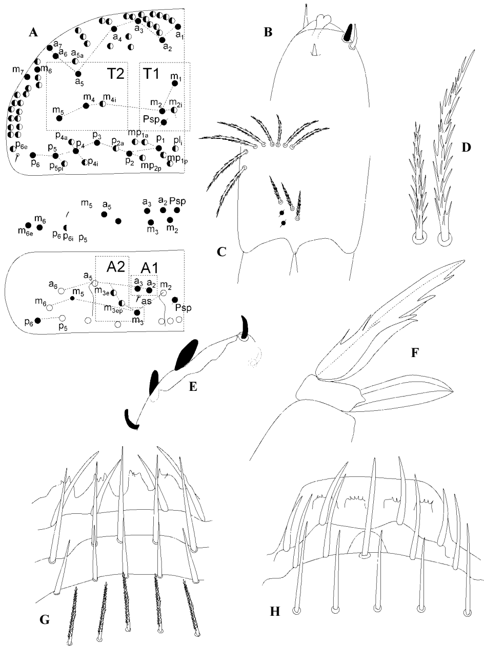
Fig. 4 E. nivalis . A chaetotaxy (thoracic tergite III, abdominal tergites I and II) of individuals from Saxony-Anhalt (Germany SMNG); B tip of antennal segment IV; C manubrial plate; D common short setae (»type five«); E sensory organ of antennal segment III; F claw and empodium; G and H labral papillae of specimens from Irati (Spain) and Norway respectively.
