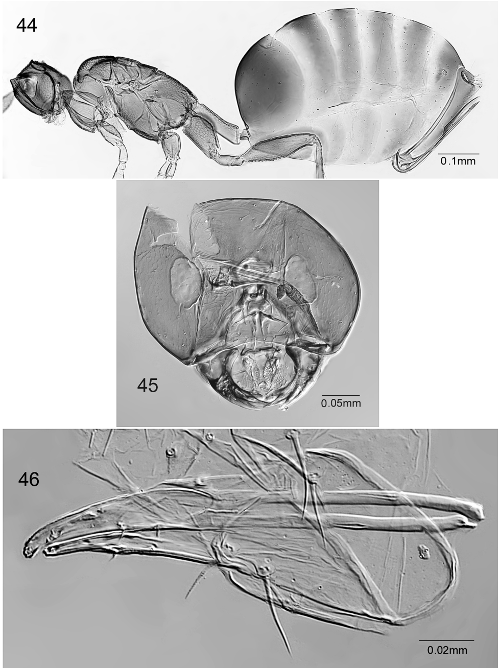
FIGURES 44–46. Eustochus spp. 44– nipponensis , body lateral (holotype); 45– aripennis , male head, anterior (Switzerland, Chancy); 46– aripennis , male genitalia, ventrolateral.
