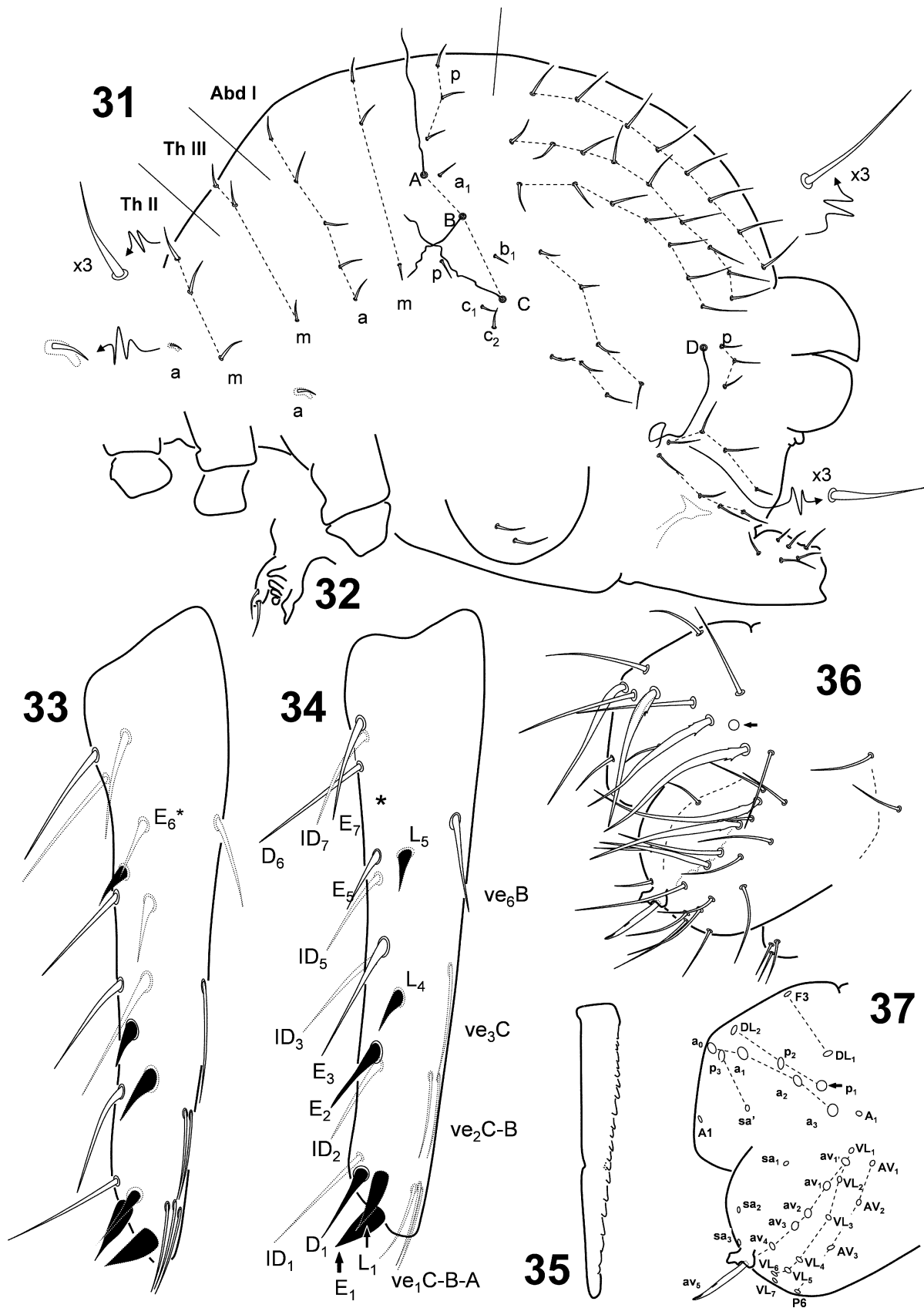
FIGURES 31–37. Pygmarrhopalites cantavetulae sp. nov.: 31, body chaetotaxy; 32, tenaculum; 33–34, dens (external view; *E 6 lacks in one of dens); 35, mucro; 36–37, Abd VI.
