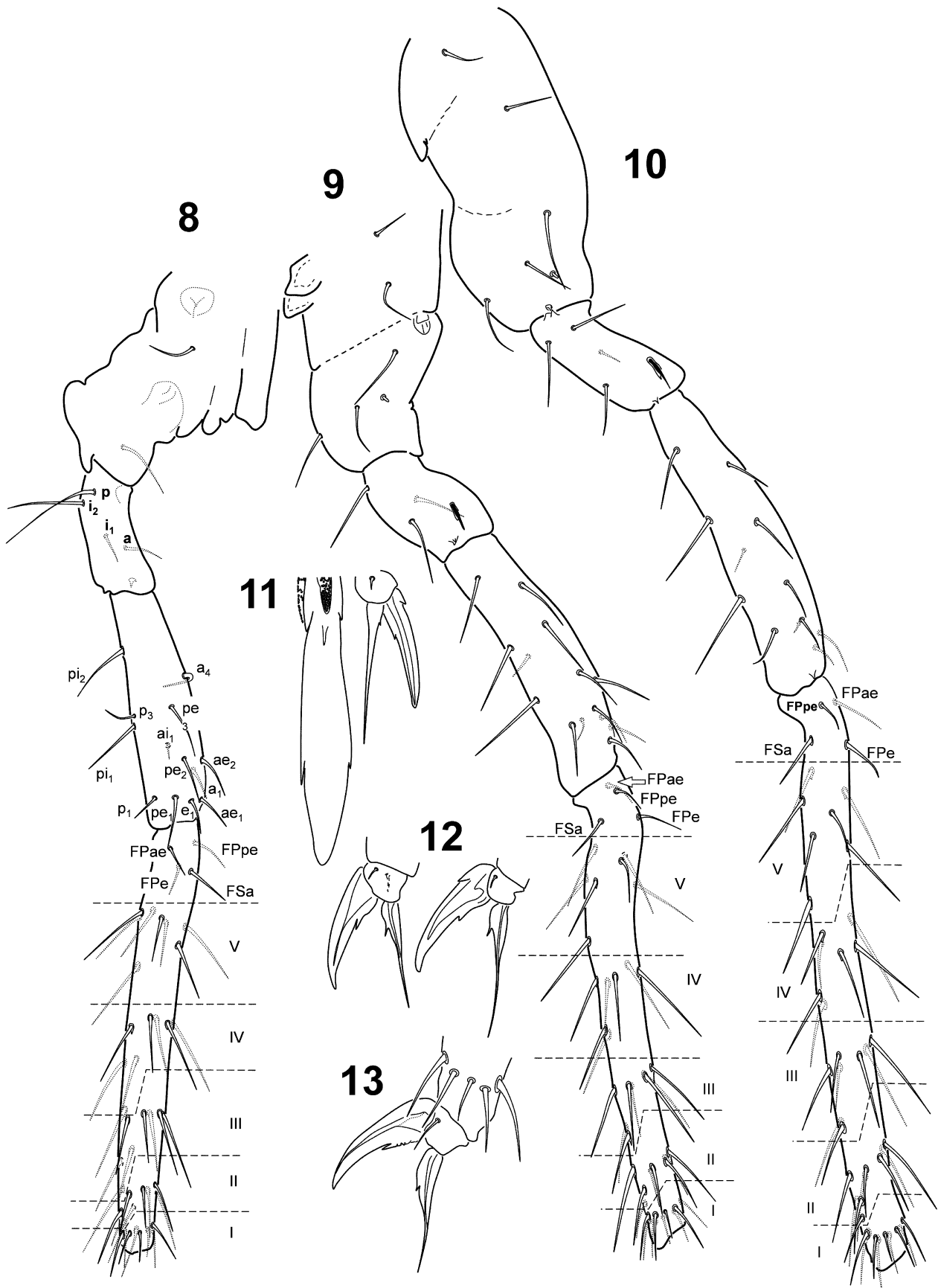
FIGURES 8–13. Pygmarrhopalites maestrazgoensis sp. nov.: 8, foreleg (posterior view); 9, midleg (posterior view); 10, hind leg (posterior view); 11, claw of foreleg (dorsal and ventro-posterior view); 12, claw of mid leg; 13, claw of hind leg.
