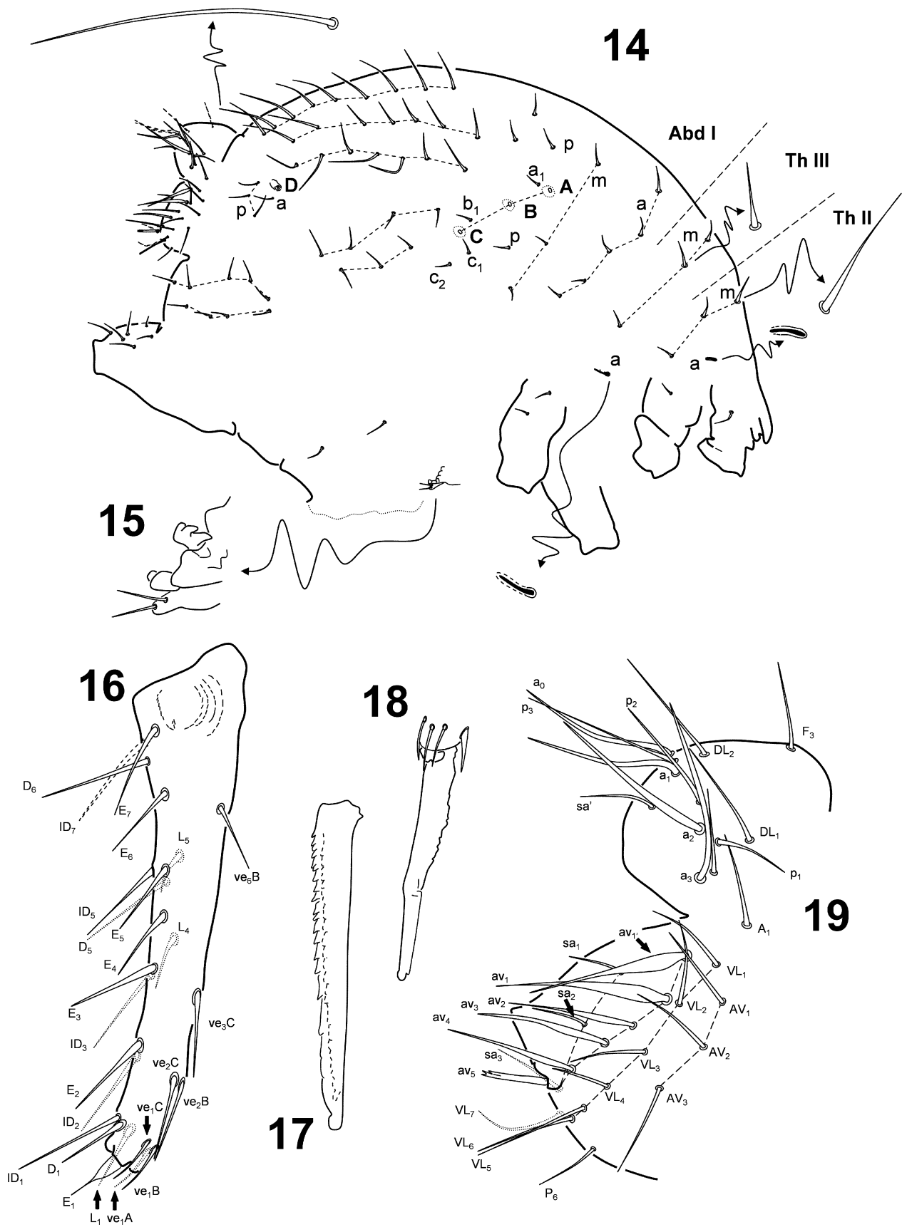
FIGURES 14–19. Pygmarrhopalites maestrazgoensis sp. nov.: 14, body chaetotaxy; 15, tenaculum; 16, dens (external view); 17, mucro (external view); 18, mucro (internal view); 19, Abd VI.
