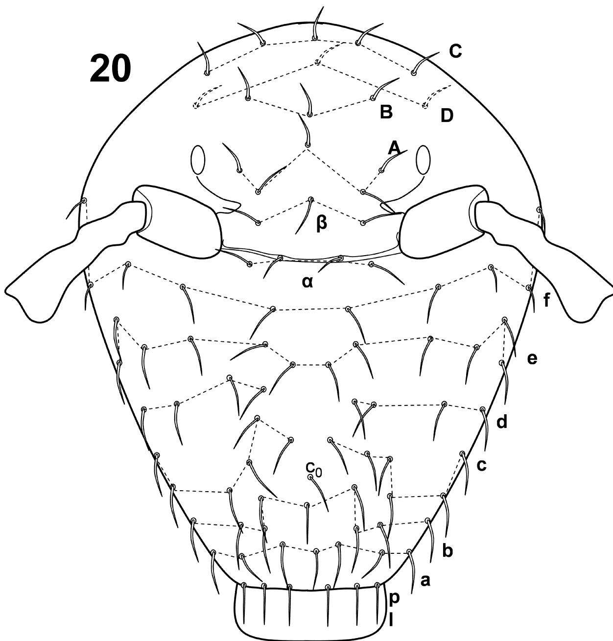
FIGURE 20. Pygmarrhopalites cantavetulae sp. nov., head chaetotaxy.
