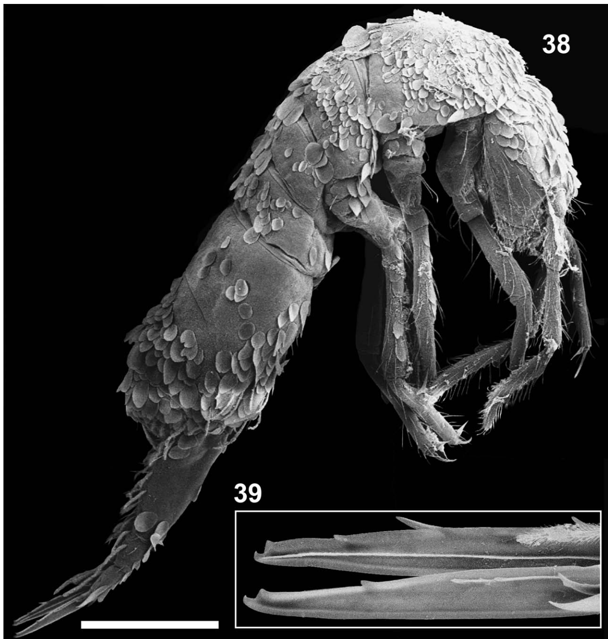
FIGURES 38–39. Oncopodura fadriquei Jordana & Baquero sp. nov. : 38, habitus at SEM microphotograph; 39, macro at SEM microphotograph.
