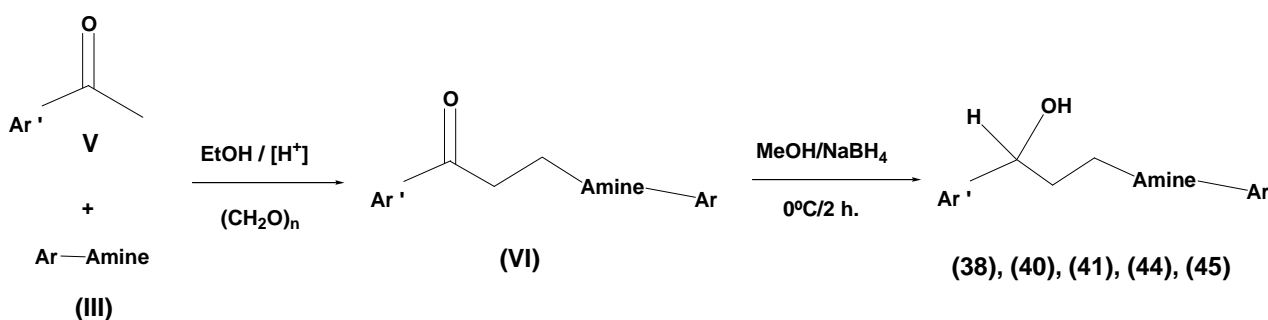
Scheme 2. Synthesis of 1-aryl-3-substituted propanol derivatives 38 , 40 , 41 , 44 and 45 .
