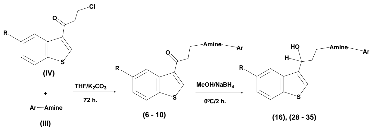
Scheme 2. Synthesis of 1-aryl-3-substituted propanol derivatives 38 , 40 , 41 , 44 and 45 .
