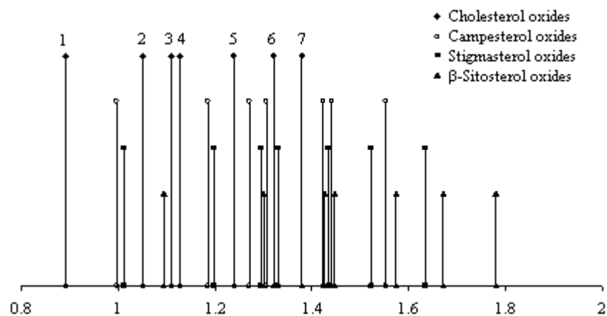
Figure 1. Representation of the relative retention times of TMS-oxysterol in relation to 19-hydroxycholesterol on VF-5ms (Varian). GC-MS and He as a carrier gas were used. The elution order of TMS-oxysterols was: (1) 7 \alpha -hydroxy, (2) 7 \beta -hydroxy, (3) 5,6 \beta -epoxy, (4) 5,6 \alpha -epoxy, (5) triol, (6) 25-hydroxy and (7) 7-keto.
