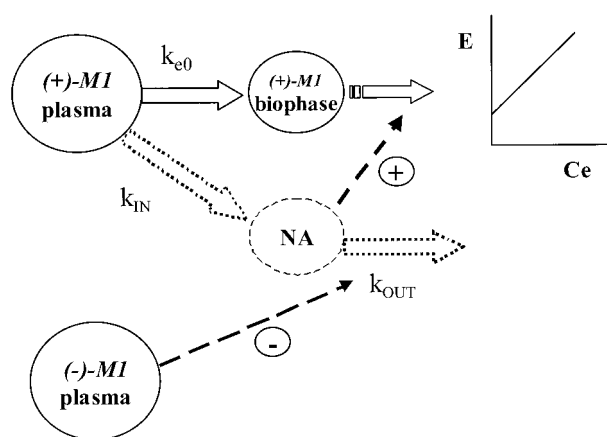
Fig. 2. Schematic representation of the pd model selected during the analysis of the in vivo interaction between (+)-M1 and (-)-M1 in the antinociceptive effect.
