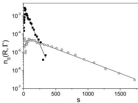
FIG. 3. Probability n_s(R, \Gamma) of finding an avalanche of size s for an orifice size R=3.02 , without vibration ( \Gamma=0 , \blacksquare ) and with vibration ( \Gamma=0.22 , \circ ). The solid lines correspond to fits using Eq. (4). For the nonvibrated silo, the fitting parameters are p=0.981 and q=0 . For the vibrated silo p=0.981 and q=0.836 .
