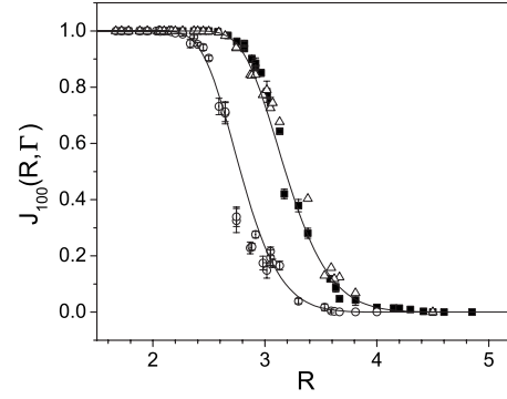
FIG. 4. Jamming probability J_{100}(R, \Gamma) , i.e., the probability that the silo gets jammed before 100 particles flow through the outlet, as a function of R , for the vibrated ( \circ ) and the nonvibrated ( \blacksquare ) silo. The lines correspond to a fit using Eq. (2). The “weak jamming” probability J_{100}^w(R) for the avalanches within an avalanche is also shown ( \triangle ).
