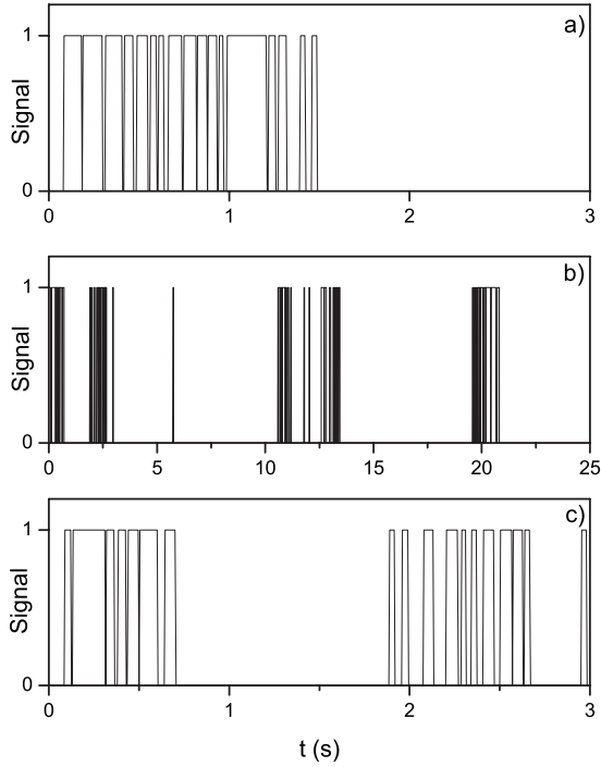
FIG. 2. Signal from the photosensor at the silo exit: a value of 1 indicates that a particle is blocking the beam, zero means that the beam is unobstructed. (a) Nonvibrated silo. (b) Vibrated silo. (c) A zoom of the signal shown in (b) during the first three seconds, the same time stretch as in (a). All the data shown have been obtained for an orifice size R=3.05 .
