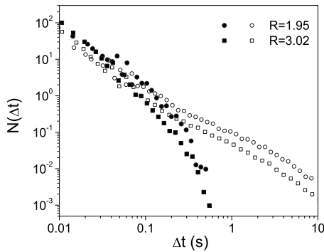
FIG. 7. Normalized histograms of the time intervals ( \Delta t ) within an avalanche during which there are no particles flowing through the orifice. Closed (open) symbols represent the data obtained with the nonvibrated (vibrated) silo for the values of R indicated in the legend. For each R , measurements have been carried out within, at least, 3000 avalanches.
