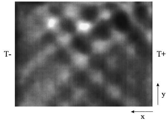
FIG. 3. Top image of the hydrothermal waves obtained by shadowgraph technique. Cold sidewall is indicated by T- and hot sidewall by T+ . Both of the two oblique waves are traveling from the cold to the hot side at the same time.
