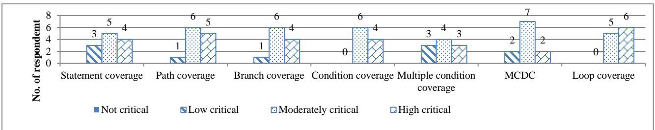
Figure 8: Weighted scoring the critical level of adopting the structural code coverage
