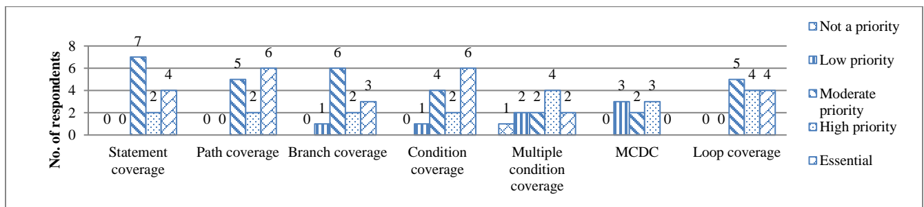
Figure 4: Level of prioritization the structural code coverage in programming assessments
