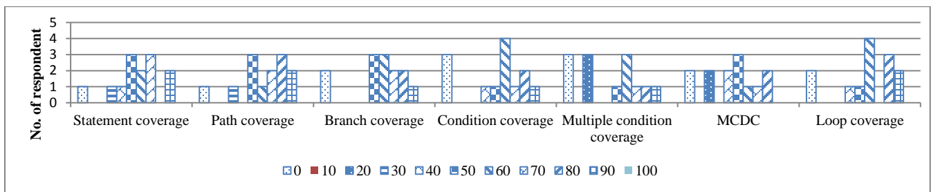
Figure 9: Scoring for each of the structural code coverage
