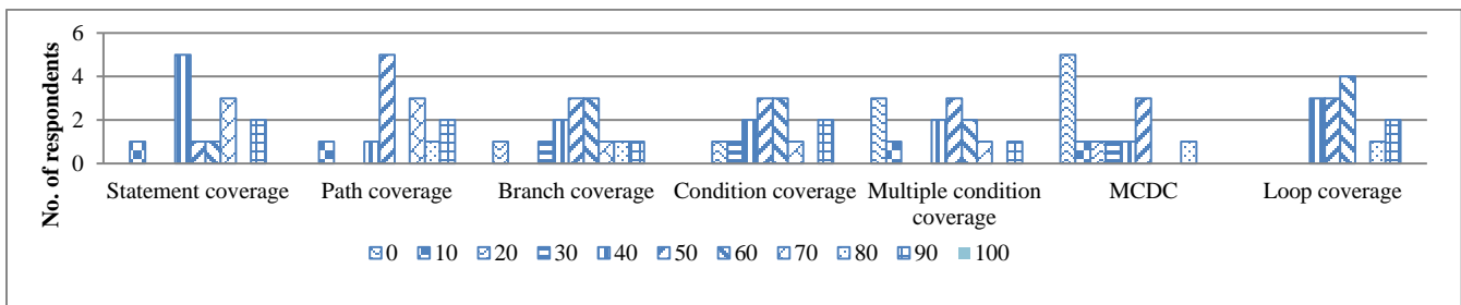
Figure 5: The current means of scoring the structural code coverage in programming assessments
