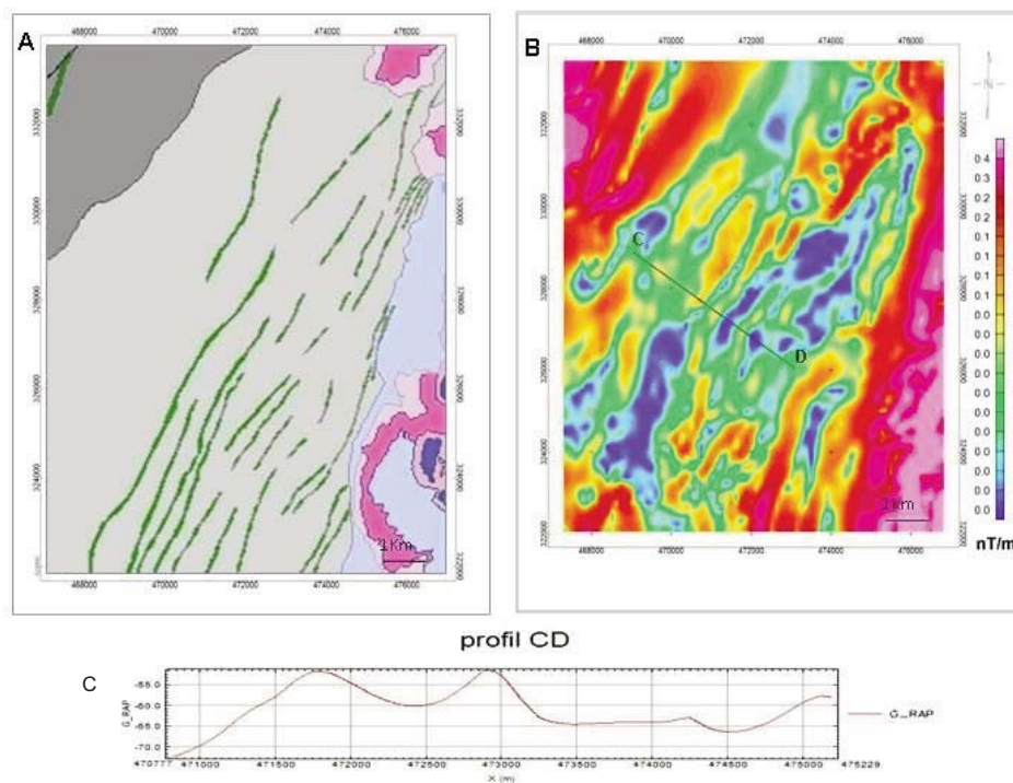
Fig. 10 A. Geological map of the sector of sills and dikes, SW of Agourai (see legend in Figure 3), B. Horizontal gradient magnetic map of the same sector (see location figure 7), C. Magnetic signal from the profile CD
