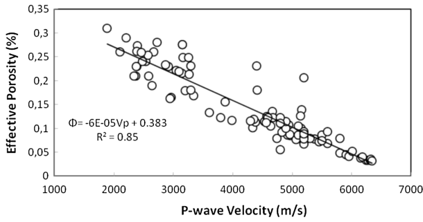
Fig. 7 Graph of effective porosity (Φ) and P-wave velocity (V p )
