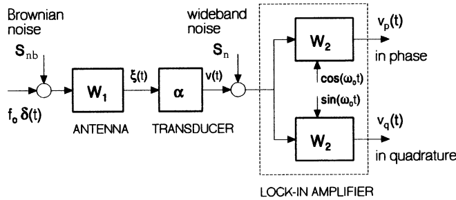
Fig. 4. – Model of antenna, transducer and lock-in amplifier. S_{nb} is the narrow-band noise spectrum at the resonance frequency of the mode and S_n is the wide-band noise spectrum.
