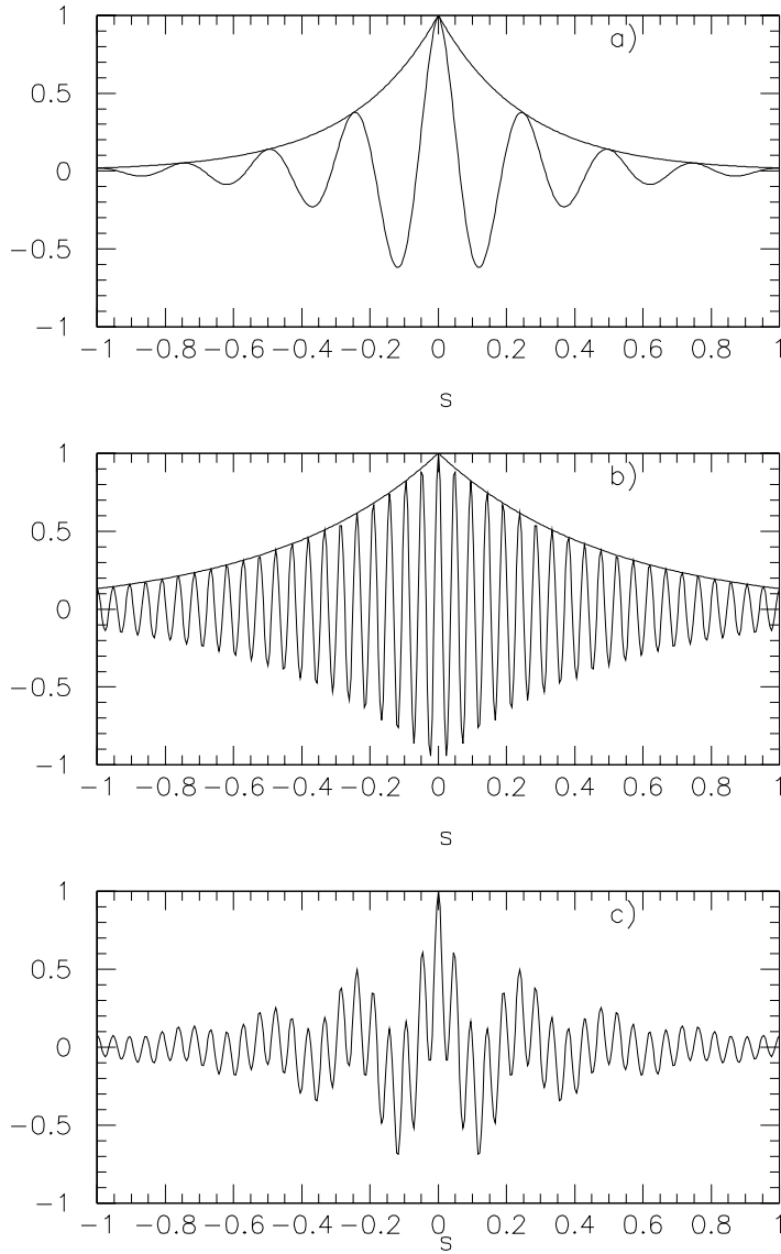
Fig. 6. - a) Same as fig. 5a), with |d'| = 4 \text{ rad s}^{-1} ; b) same as fig. 5b), with |d'| = 2 \text{ rad s}^{-1} ; c) Same as fig. 5c), with |d'| = 4 \text{ rad s}^{-1} , |b'| = 2 \text{ rad s}^{-1} : here the envelope is not a simple exponential.
