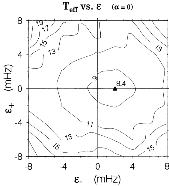
Fig. 24. - Loss of the filter performance due to errors in the resonance frequencies. Dependence of the effective temperature (expressed in mK) on the frequency errors \epsilon_- and \epsilon_+ for \alpha = 0 .
