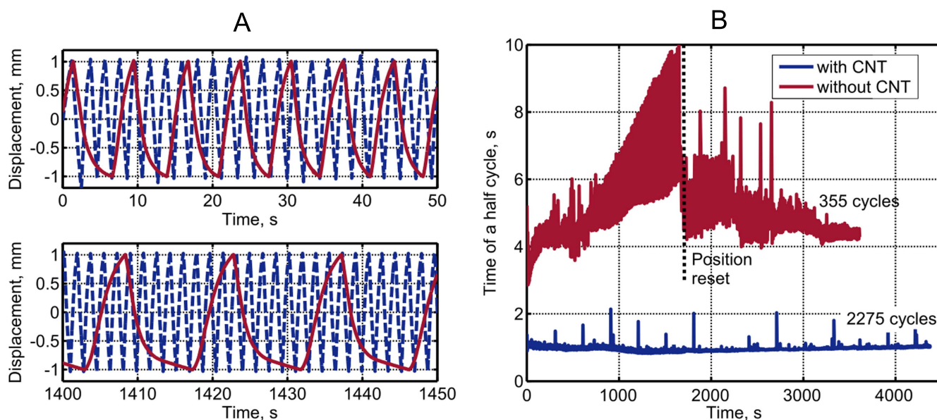
Figure 5. (A) Bending profiles versus time for actuators with (blue dotted line) and without (red line) CNTC. The voltage polarity ( \pm 1.5 V) was changed every time the actuator reached the \pm 1 mm set value. (B) Time needed for the tip of the actuator to move from to \pm 1 mm from its initial position vs time for the CNTs (blue) and simple (red) actuators. \pm 1.5 V was used to change the direction of bending as soon as the actuator tip reached the set value. For the actuator without CNTC the value was reset to -0.8 mm and +1.2 mm due to the large creeping (shown as dotted line).
