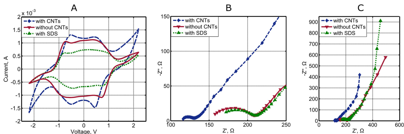
Figure 4. (A) CV voltammogram of actuators without CNTC (red full line), with CNTC (blue dashed line) and with SDS (green dotted line) ( 20 \text{ mV s}^{-1} scan rate). (B)–(C) Nyquist plots for PEDOT:PSS with and without CNTC measured without prior bias potential from 100 kHz to 10 mHz.
