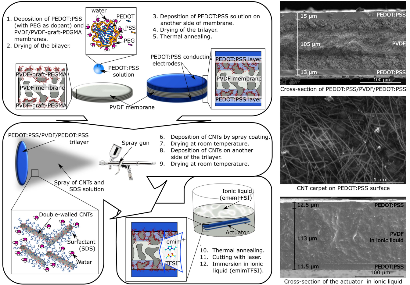
Figure 1. Illustration of the main fabrication steps of PEDOT:PSS/PVDF/PEDOT:PSS actuators with sprayed CNT carpets. Insets show assumed morphology of PEDOT:PSS secondary-doped with PEG structure in solution, PVDF/PVDF-graft-PEGMA/PVDF hybrid membranes (produced as in [41]), CNT and SDS organisation in aqueous solution and molecular structure of the ionic liquid. SEM images of the cross-sections of the actuators on the right show the structure of the actuators in dry state, after immersion in ionic liquid and the surface of PEDOT:PSS with sprayed CNT carpet (CNTC).
