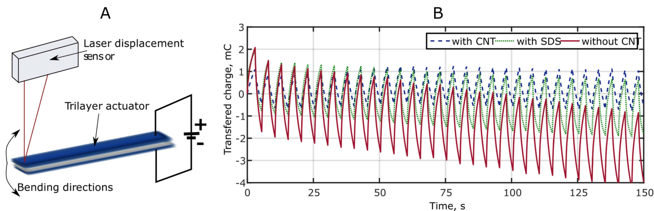
Figure 2. (A) Schematic illustration of the set-up used for actuation characterization by laser displacement sensor. (B) Calculated transferred charge during actuation of trilayer actuators with and without post-treatments. A 1.5 V square wave was used for actuation.
