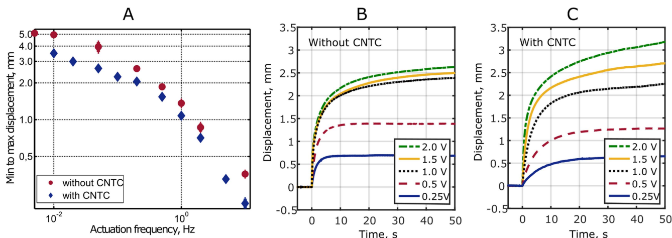
Figure 3. (A) Frequency response of actuators with and without CNTs. Calculated after actuation with a 1.5 V square wave as an average of at least three cycles. (B) Open loop step response of actuators without CNTC at different voltages. (C) Open loop step response of actuators with CNTC at different voltages.
