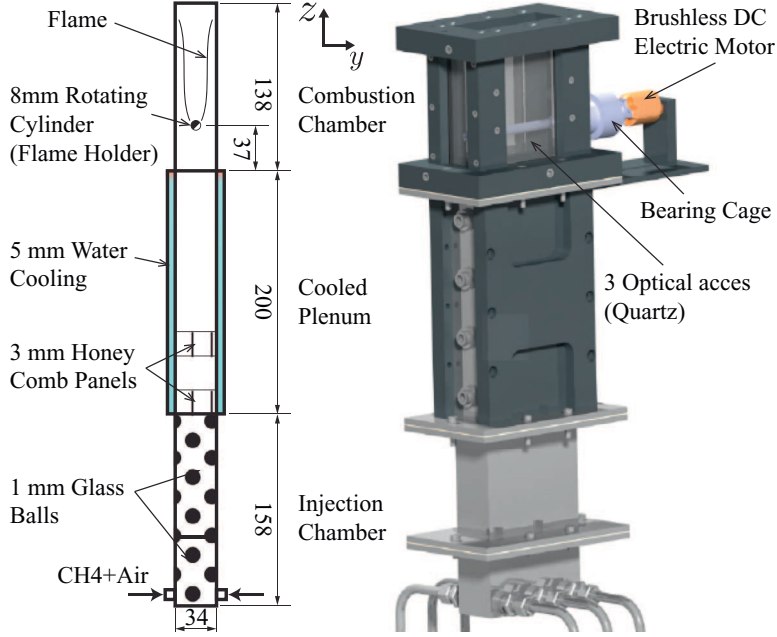
Fig. 2. Transverse cut ( left ) and isometric view ( right ) of the Intrig burner.
