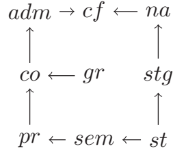
Figure 2. Extension Inclusion Graph Inc(\mathcal{S})
