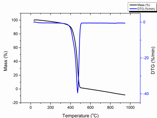
Figure 1 TG/DTG for virgin LDPE powder.
