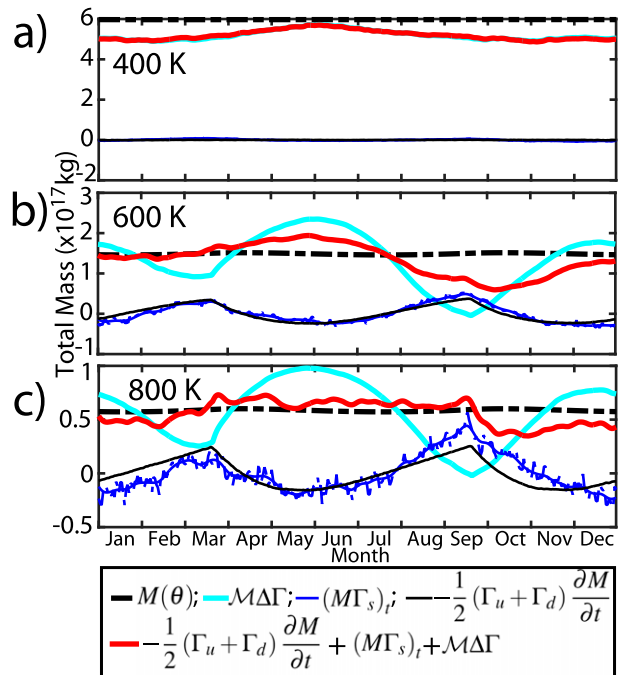
FIG. 5. Twenty years of model output have been averaged for each day of the year to produce a climatological seasonal cycle for the different terms in the age budget: M(\theta) = M\Delta\Gamma + (M\Gamma_s)_t + [-(\Gamma_u + \Gamma_d)M_t/2] . Each panel shows the individual terms and the right-hand side at a different level: (a) 400, (b) 600, and (c) 800 K.
