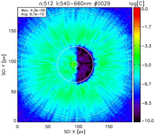
(a) PICTURE-C broadband image plane contrast map showing the contrast provided by the VVC and a dark hole created by thirty iterations of EFC. This contrast map corresponds to the simulated science image corrected for spatial variations in VVC transmission divided by the peak pixel value of a simulation of the same system with the VVC element removed. 12
