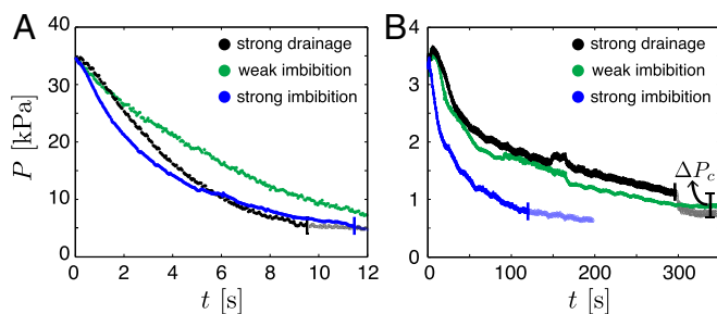
Fig. 5. Evolution of the injection pressure during strong drainage, weak imbibition, and strong imbibition at (A) Ca = 2.9 \times 10^{-1} and (B) Ca = 2.9 \times 10^{-2} . The pressure measurements are shifted in time so that t = 0 s is the time when the invading water first enters the flow cell. The end of each experiment (i.e., the time when the water first reaches the perimeter of the flow cell) is marked with a vertical line and subsequent measurements are translucent. (B) The sudden drop in injection pressure as the water exits the flow cell in strong drainage corresponds to the capillary pressure \Delta P_c across the oil–water interface.
