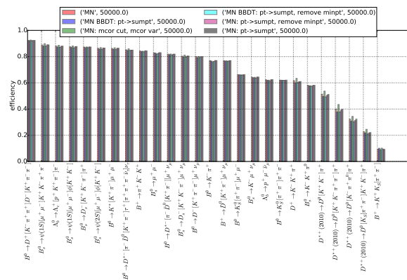
Figure 8. Efficiencies comparison for MatrixNet: with corrected mass, without it (MN), with the scalar sum of transverse momentum (sum pt , without min and vector pt ). These models were ‘converted’ to BBDT format and compared. The output rate is set to 50 kHz.
