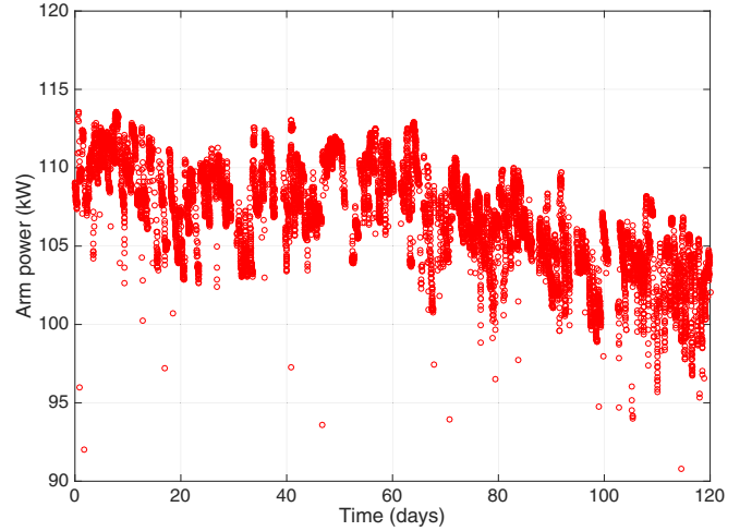
FIG. 2. Optical power resonating in the LIGO Livingston interferometer (L1) during the first science run. The power was fluctuating by a few percents, and slightly decreased by the end of the run due to the drift of the input power.
