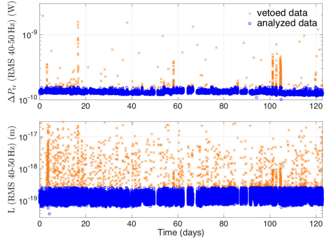
FIG. 8. Data quality cut. The quality of the data is estimated based on the rms of the signal computed between 40 and 50 Hz. Red points are subtracted from the analysis.
