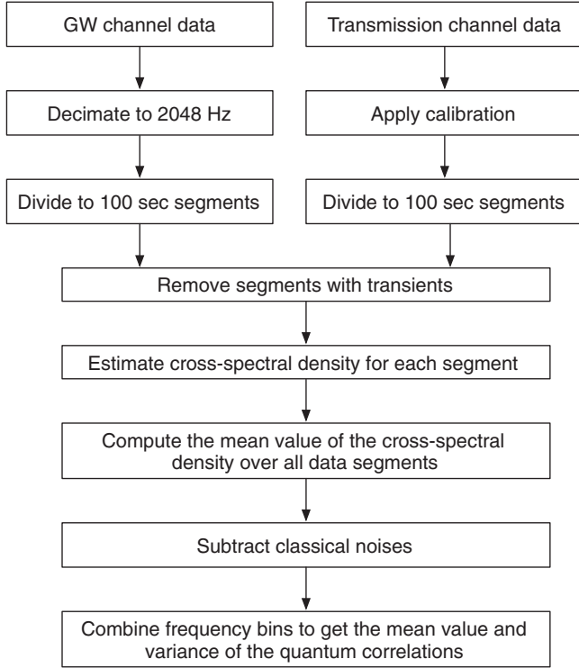
FIG. 7. Data analysis flow diagram for the estimate of the quantum correlations.
