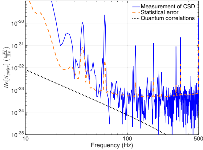
FIG. 9. Cross-spectral density between the GW channel and the differential transmission channel computed using O1 data. The orange (dashed) trace shows the square root of the variance at each frequency bin. The black (dotted) line shows the mean value of the theoretically predicted quantum correlations.
