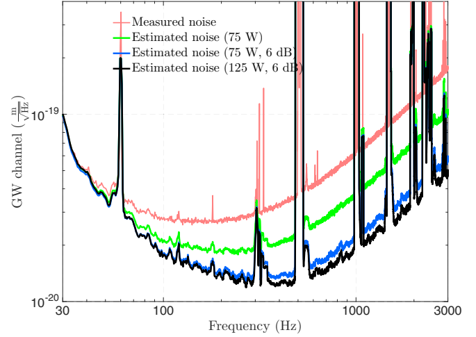
FIG. 5. Estimated noise spectra of LIGO interferometers for future science runs when the input power is increased and squeezed states of light are introduced.
