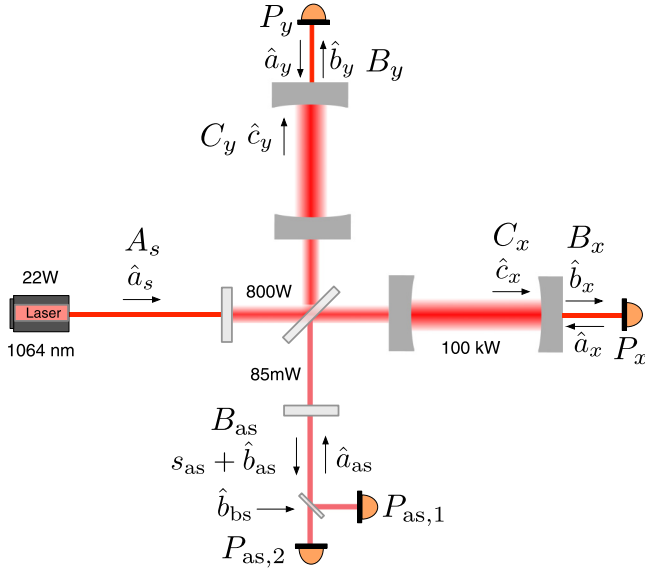
FIG. 1. Layout of an Advanced LIGO detector. The annotations show the optical power in use during O1. Also shown are vacuum and laser fields entering the interferometer through the input, output, and transmission ports. The GW signal s_{as} (also includes classical noises) leaves the interferometer through the antisymmetric port.
