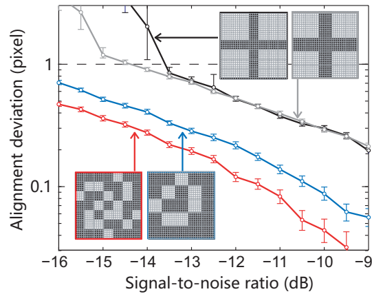
FIG. 5. (Color Online) The “horizontal” alignment deviation is shown for the four alignment marks under various signal-to-noise ratios. The vertical deviation is almost identical. The color of each plot line borders the corresponding marker. All markers have been expanded to 35 by 35 pixels to illustrate the idea of pixel expansion. The top, black line, on the right edge, corresponds to the 7 by 7 cross, while the second to top, grey line corresponds to the 5 by 5 cross. The second to bottom, blue line corresponds to the optimal 5 by 5 marker, while the bottom, red line corresponds to the optimal 7 by 7 matrix.
