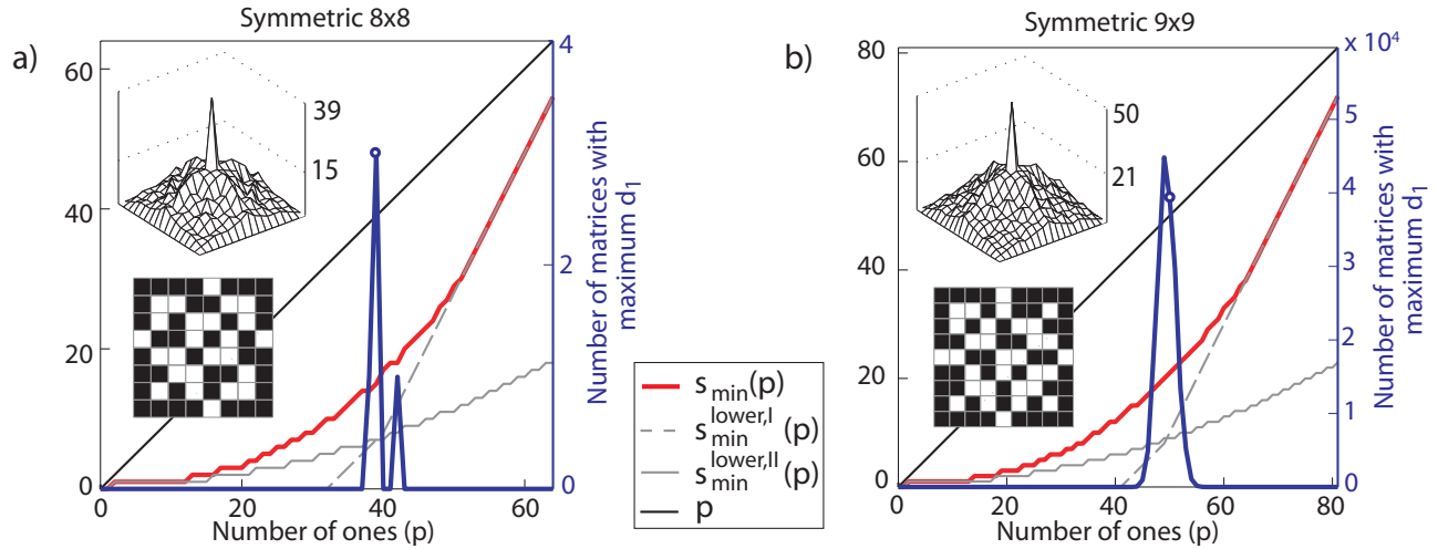
FIG. 4. (Color Online) Results of the exhaustive searches for diagonally-symmetric 8 by 8 and 9 by 9 matrices.
