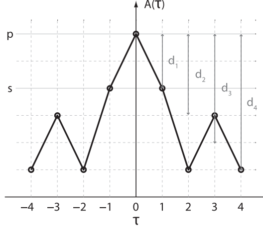
FIG. 1. (Color Online) We illustrate an autocorrelation function A(\tau) , whose peak value is p , highest sidelobe value is s , and whose peak-sidelobe distances are d_i .
