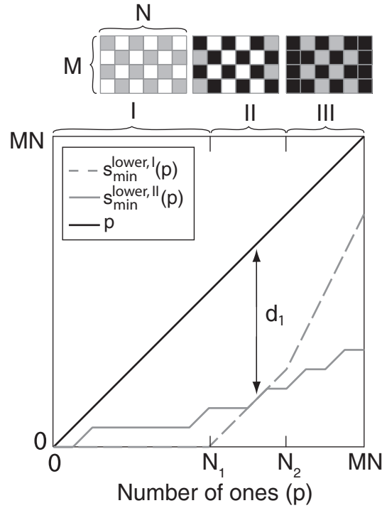
FIG. 2. (Color Online) Lowerbounds of s_{\min}(p) , s_{\min}^{\text{lower,I}}(p) and s_{\min}^{\text{lower,II}}(p) . p is the autocorrelation peak. The three matrices on top illustrate the methods of filling black pixels for regions I, II and III for the matrix construction of s_{\min}^{\text{lower,I}}(p) . The grey pixels show spots to be filled in that region, while the black pixels are spots that have been filled in previous regions.
