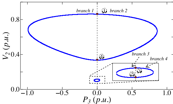
Fig. 21: P_3V_2 curves
