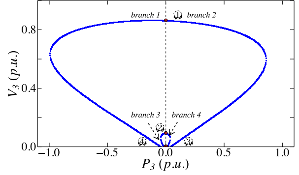
Fig. 22: P_3V_3 curves
