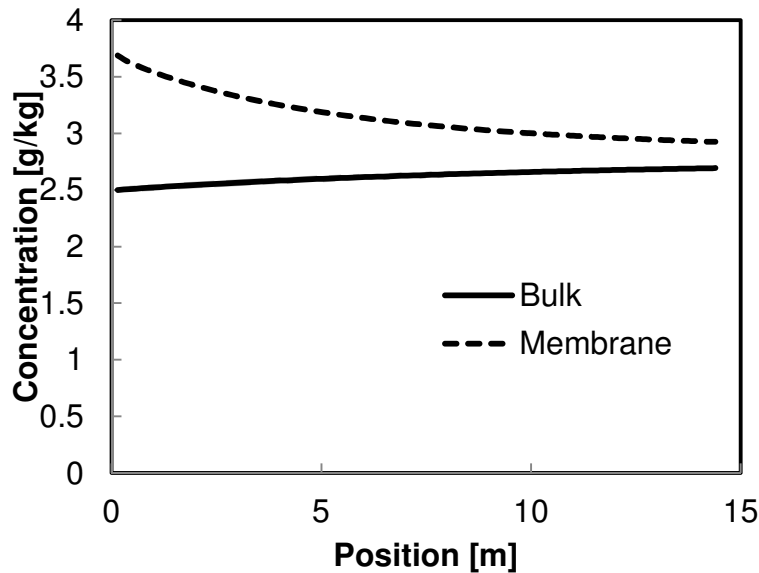
Figure 16. Modeled \text{CaSO}_4 concentration profiles across a long MD module.
