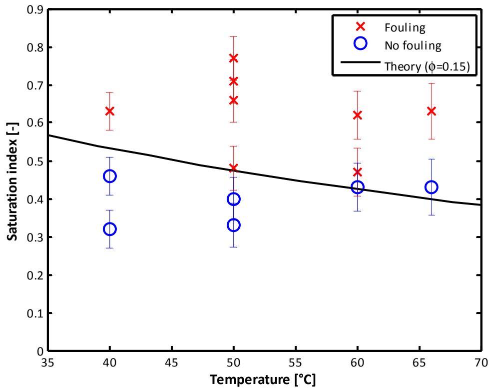
Figure 10. Experimental fouling regime map overlaid with the theoretical prediction for \text{CaSO}_4 at varied temperature and salinity at a single flow rate (0.314 m/s). Permeate flux varied from 7.5-30 \text{kg/m}^2\text{-hr} as temperature increased.
