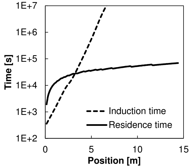
Figure 9. Induction time and residence time along the length of a full-scale MD module with 2.5 g/kg \text{CaSO}_4 at the inlet. Where residence time exceeds induction time, nucleation and fouling can be expected.
