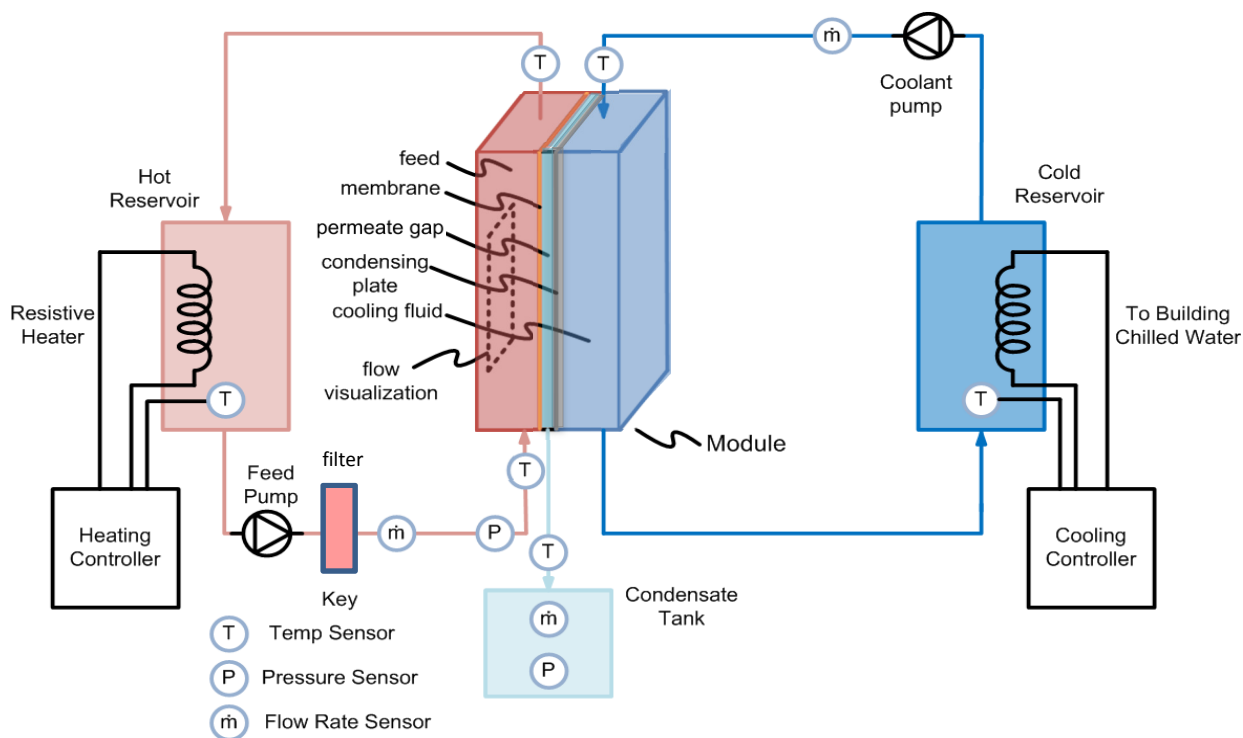
Figure 4. Schematic diagram of the fouling apparatus (figure from [6]). The permeate gap MD module has two flow loops for the hot saline feed and cooling fluid.
