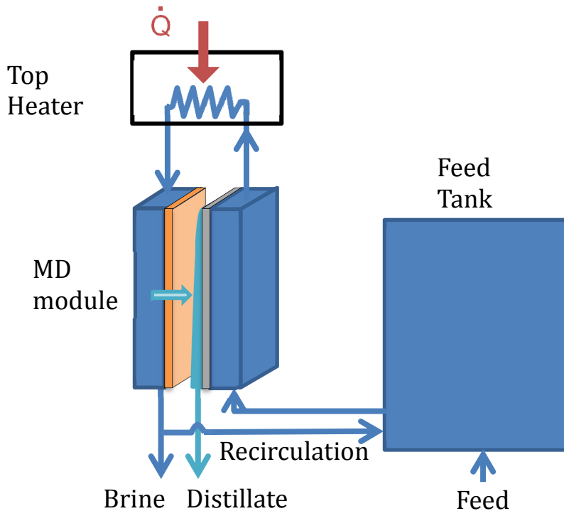
Figure 17. Schematic diagram of membrane distillation with brine recirculation.
