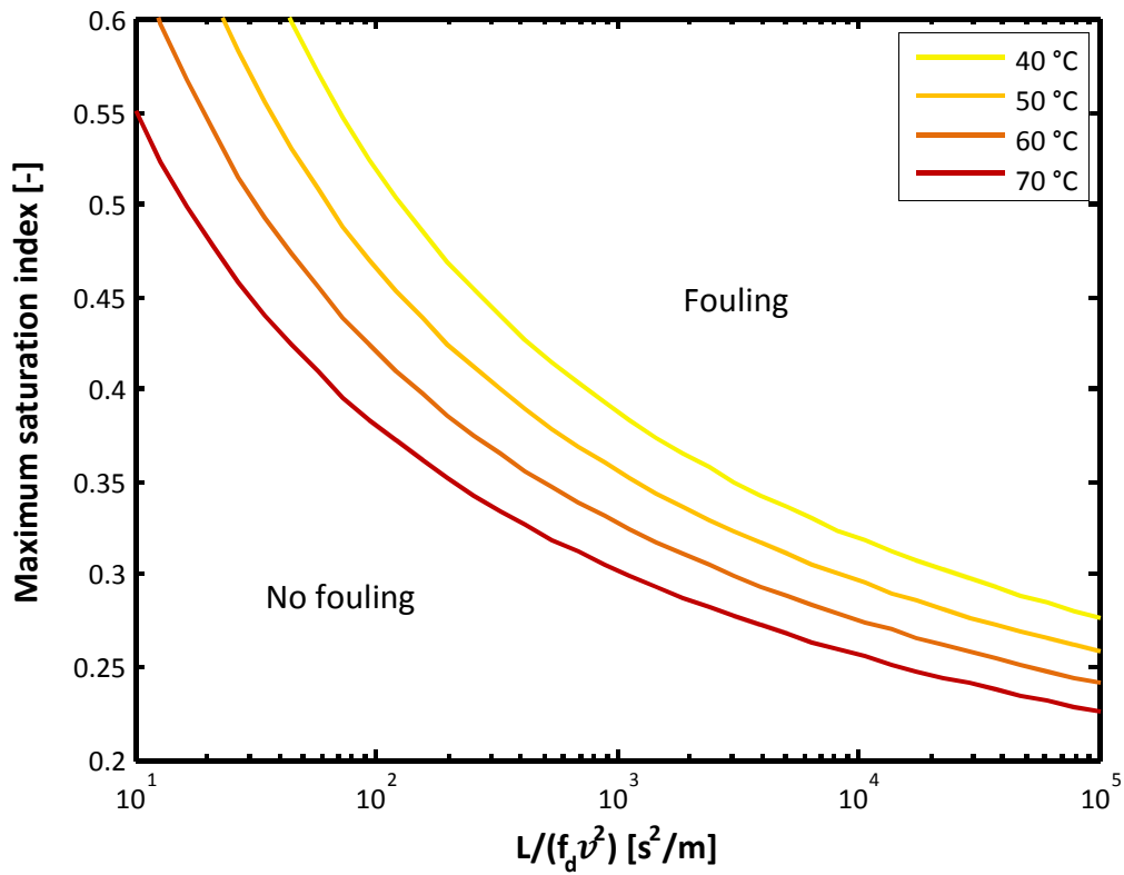
Figure 13. Universal CaSO 4 fouling regime map: at saturation indices above the curve for a given temperature, systems are prone to fouling according to the present model. The horizontal axis incorporates membrane length L , Darcy friction factor f_d , and bulk velocity v . The incorporation of f_d collapses laminar and turbulent flow regimes into the same curve.
