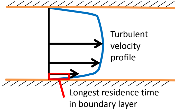
Figure 1. The maximum residence time in the system occurs in the boundary layer near the membrane.
