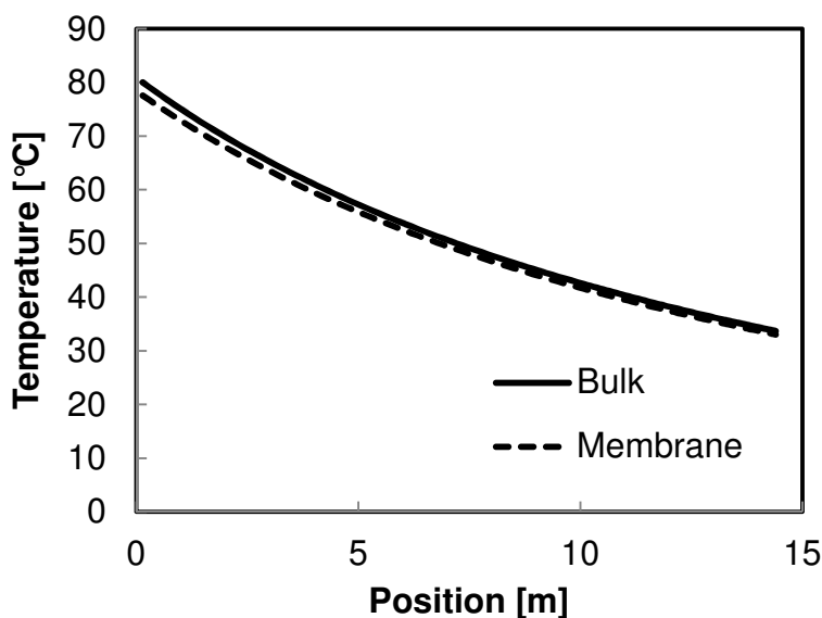
Figure 15. Modeled feed temperature profiles across a long MD module.
