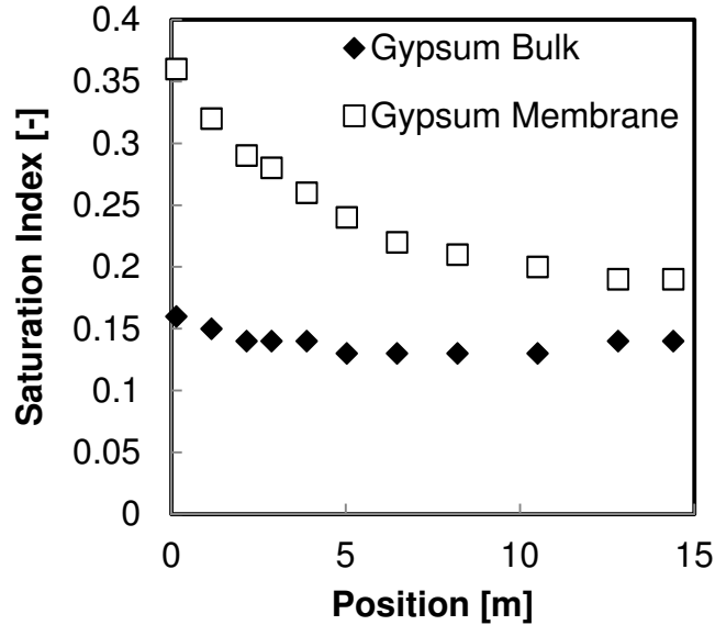
Figure 8. Calculated saturation index of gypsum at the membrane surface and in the feed bulk solution across an MD module of representative industrial length L = 14.4 m, width = 0.5 m, channel depth = 1 mm, and feed velocity = 0.23 m/s [45, 46]. For this system, the bulk temperature at the entrance was 80 °C and dropped to 34 °C at the feed exit. The concentration of \text{CaSO}_4 in the feed inlet is 2.5 g/kg, and the overall system flux is 4.2 kg/m 2 -hr.
