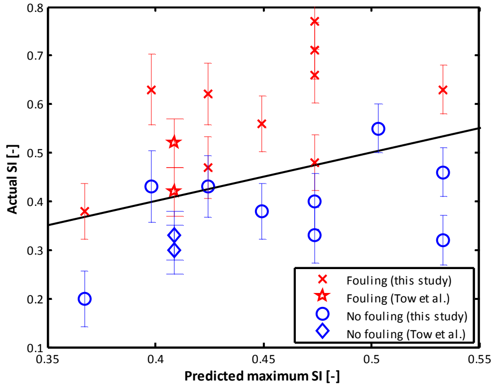
Figure 12. Validation of model using all present measurements plus data collected from a different MD module by Tow et al. [48].
