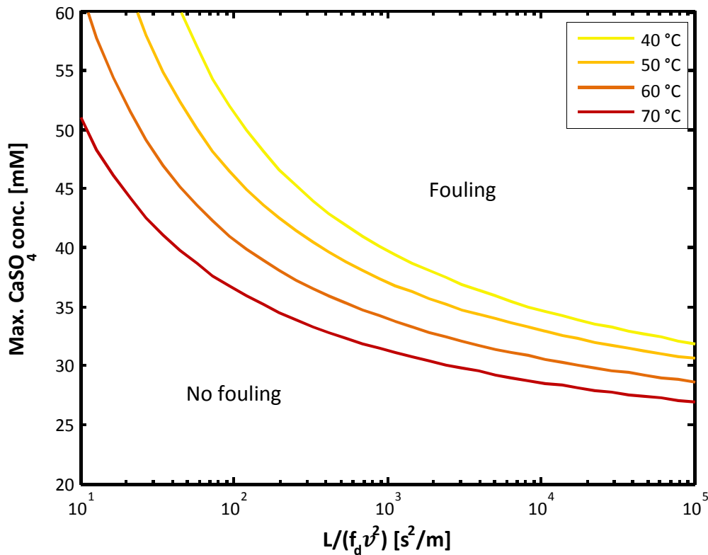
Figure 14. Universal CaSO 4 fouling regime map given in terms of concentration: at concentrations above the curve for a given temperature, systems are prone to fouling according to the present model.
