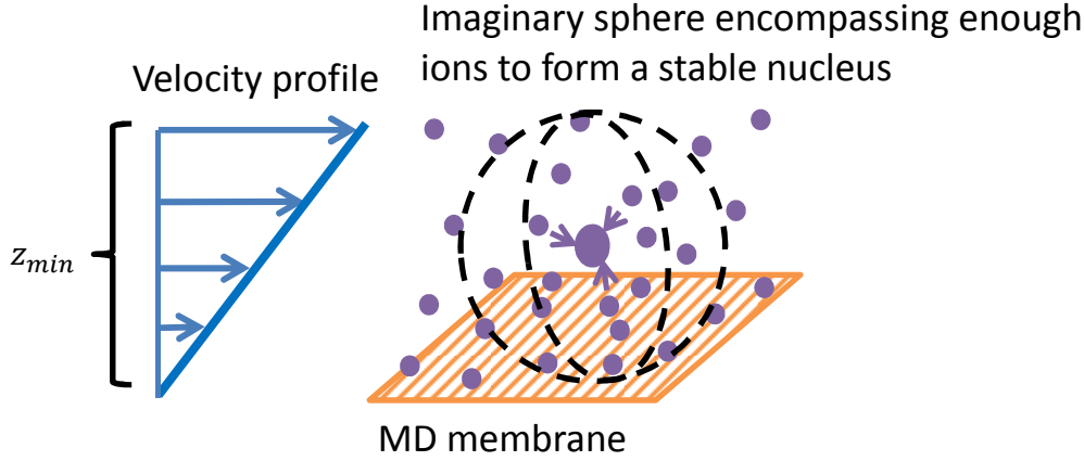
Figure 2. The flow profile and distance z_{min} can be used to calculate the residence time. z_{min} is the distance from the wall that encompasses enough ions to form a stable nucleus.
