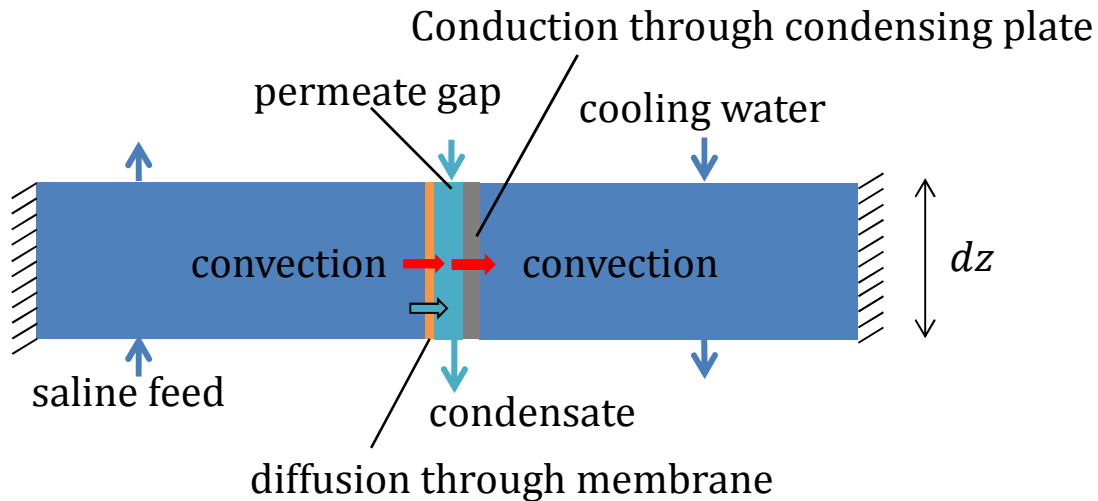
Figure 5. Computational cell for model of heat and mass transfer in membrane distillation [6, 38]
