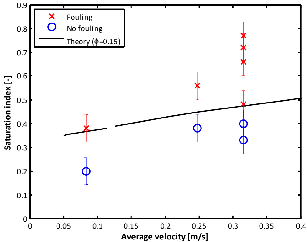
Figure 11. Experimental fouling regime map overlaid with the theoretical prediction for \text{CaSO}_4 at 50\text{ }^\circ\text{C} and three feed velocities. The break in the theoretical threshold represents the transition region between laminar and turbulent flow in the channel. Permeate flux varied from 18.0\text{-}19.2\text{ kg/m}^2\text{-hr} for the tests at 0.08 and 0.32\text{ m/s} and about 8\text{ kg/m}^2\text{-hr} for the tests at feed velocity of 0.24\text{ m/s} where a transparent sapphire condensing surface with lower thermal conductivity was used.
