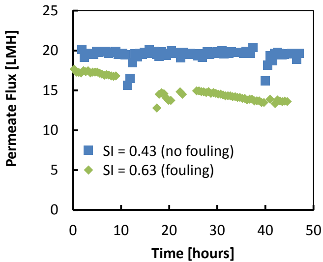
Figure 6. Permeate flux in trials at 66 °C, 0.315 m/s.
