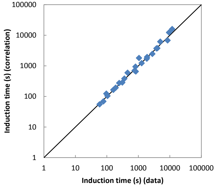
Figure 3. Fit (Eq. (13)) of gypsum induction time data by Alimi and Gadri [25].
