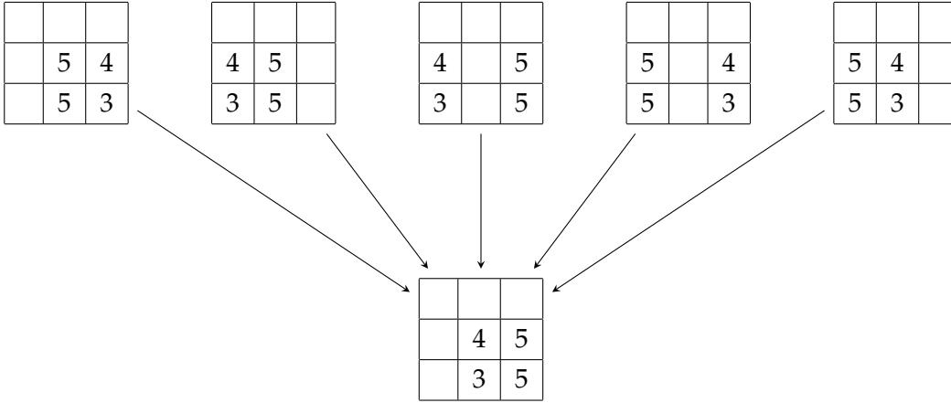
Figure 7: “Abstraction” procedure
