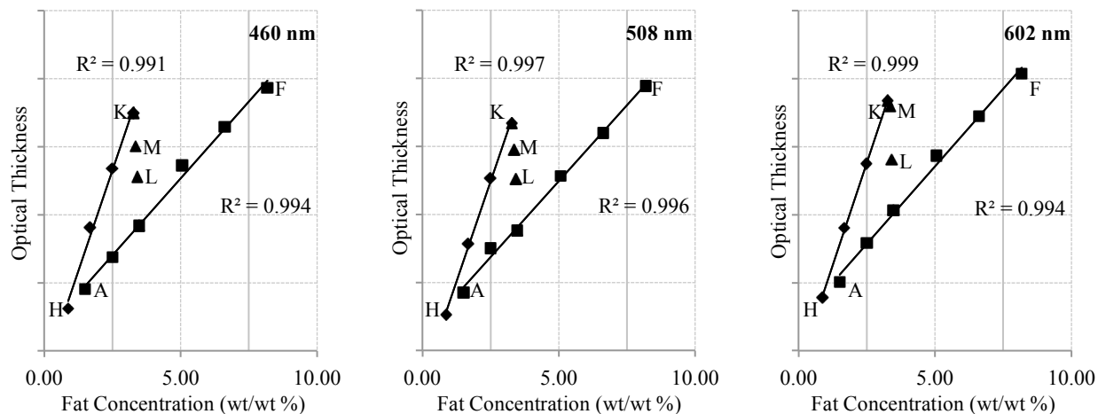
Figure 8. Estimated optical thickness \tau , in relative units, compared to the reference fat concentrations for all samples at LED wavelengths: 460 nm (a - left); 508 nm (b - center); 602 nm (c - right)
