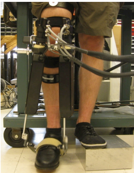
Figure 1. The Anklebot and knee brace were attached on a subject in the standing position with the dominant foot clear of the ground.
