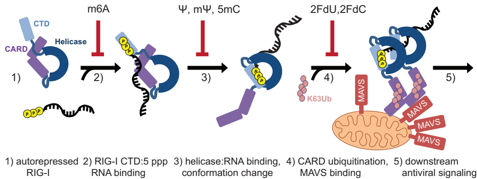
FIG 5 Model of RIG-I interaction with RNAm6A and RNAm6A . (Step 1) RIG-I is in an autorepressed conformation in the absence of ligand. (Step 2) 5' ppp RNA binds the RIG-I CTD. RNAm6A binds RIG-I with lower affinity than RNAm6A . (Step 3) The RIG-I helicase domain binds the RNA, triggering a protein conformational change. RNAs containing \Psi , m\Psi , or 5mC fail to induce RIG-I conformational change. (Step 4) The released CARDs of the activated RIG-I:RNA complex are ubiquitinated and signal downstream. This process is hypothesized to be inefficient for RIG-I:RNA2 FdN , possibly due to ATPase negative regulation of RNA binding. Ubiquitinated RIG-I induces MAVS aggregation on the surface of the mitochondria. (Step 5) Mitochondrial complexes mediate downstream antiviral signaling. Among the RNAs tested, we observed that only RNAm6A triggered RIG-I antiviral signaling.
