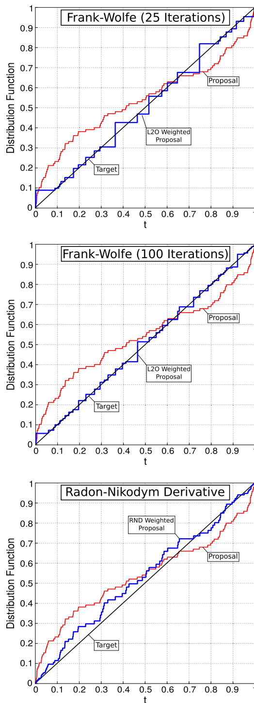
Fig. 2 Our empirical importance weights are determined using the Frank–Wolfe algorithm with step length \alpha = 2/(2+k) and premature termination. We use n = 100 proposal random samples generated from a beta distribution function (i.e., \mathcal{B}(0.5, 0.5) ) and the target is the uniform distribution function (i.e., \mathcal{U}(0, 1) ). Terminating the Frank–Wolfe algorithm after 25 iterations ( top ) results in a sparse empirical importance weight vector. Terminating the Frank–Wolfe algorithm after 100 iterations ( center ) results in a dense solution and a more accurate representation of the target distribution function. For comparison, the Radon–Nikodym importance weighted empirical proposal distribution function is provided in the ( bottom ) plot
