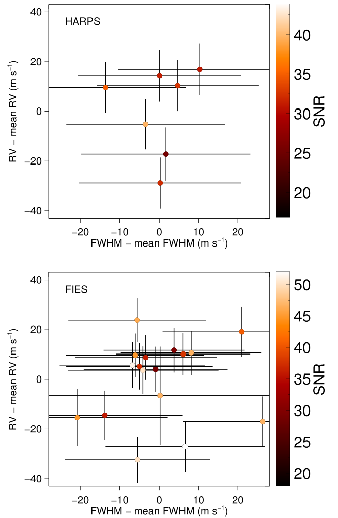
Figure 8. Full-width at half maximum (FWHM) from HARPS (top) and FIES (bottom) CCFS are plotted vs. the stellar RVs. The color code indicates the signal-to-noise ratio in the stellar spectra obtained around a wavelength range of 5560 Å. There is no evidence for correlations. The mean FWHM values for HARPS and FIES are 6,813 \text{ m s}^{-1} and 11,552 \text{ m s}^{-1} , respectively.
