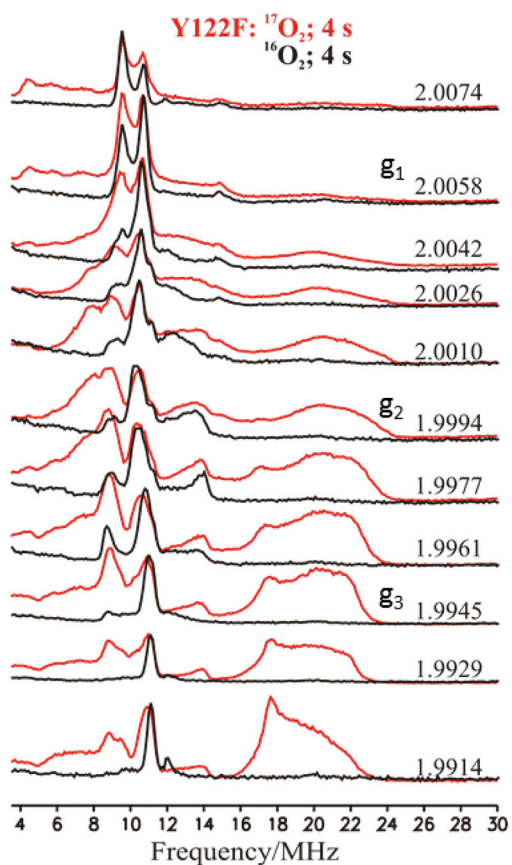
Figure 7. 2-D field-frequency plot of Davies ENDOR of X(Y122F) prepared with natural abundance (black solid lines) and 89 % ^{17}\text{O}_2 quenched at 4 s (red solid lines). Conditions: \pi pulse length = 80 ns, \tau = 600 ns, repetition time = 50 ms, T_{\text{rf}} = 40 \mu\text{s} , average microwave frequency = 34.96 GHz, T = 2 K.
