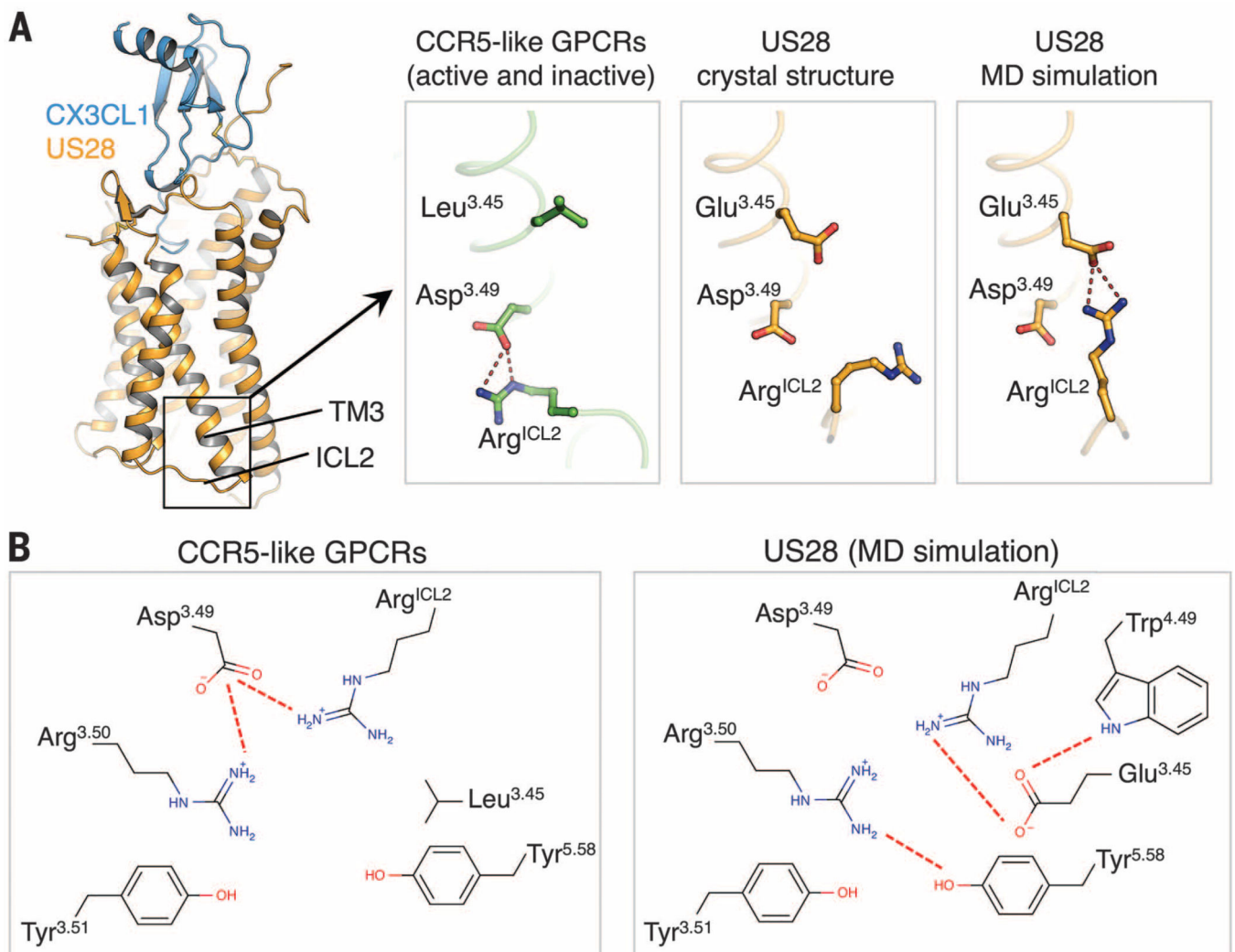
Fig. 6. Structural basis for the constitutive activity of US28 (A) Conformations of Arg ICL2 in CCR5 (green; PDB ID: 4MBS; left), the US28 crystal structure (orange; center) and the US28 MD simulations (orange; right). (B) Schematic diagram of the network of side-chain interactions surrounding the DRY motif in CCR5 (left panel) and US28 (MD simulation; right).
