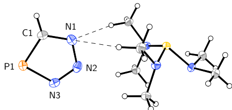
Figure 5. Molecular structure of [TAS][HCPN 3 ] shown with 50% probability thermal ellipsoids. Selected interatomic distances [Å] and angles [°] for \text{HCPN}_3^- : C1-P1 1.7216(12), P1-N3 1.6838(11), N2-N3 1.3279(15), N1-N2 1.3465(15), C1-N1 1.3400(16); C1-P1-N3 89.54(6), P1-N3-N2 111.97(8), N3-N2-N1 114.90(10), N2-N1-C1 111.56(10), N1-C1-P1 112.03(9).
