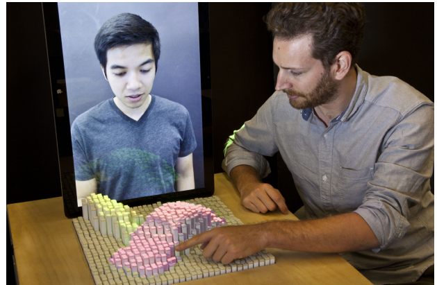
Figure 1. Physical Telepresence provides physical embodiment, remote manipulation and new capabilities through computer-mediated teleoperation. Here, local and remote users physically interact with a 3D car model.
