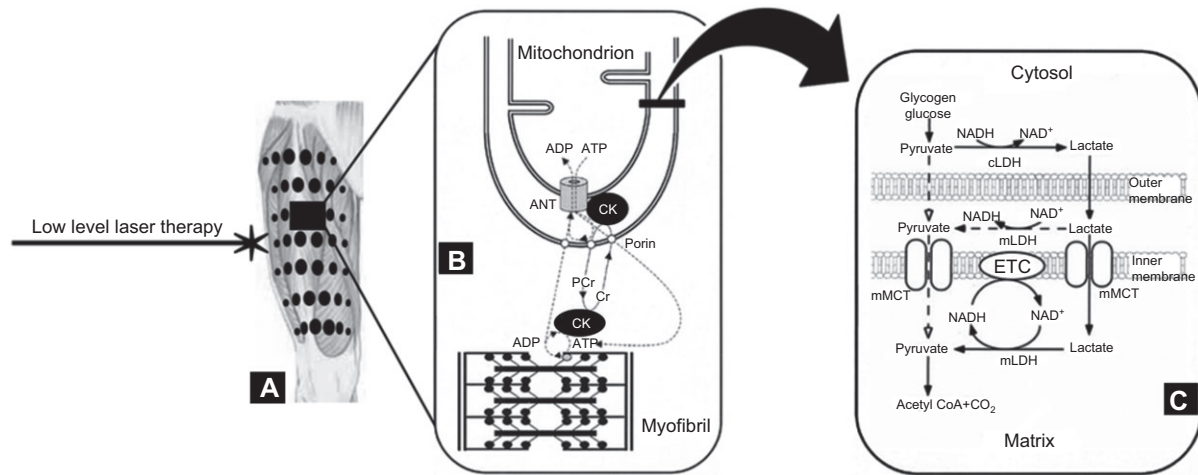
Figure 2 Based on reference [32]: (A) LLLT radiation points on femoral quadriceps muscle. (B) Mitochondrial creatine shuttle mechanism. (C) Lactate oxidation by mitochondrial pathway.
