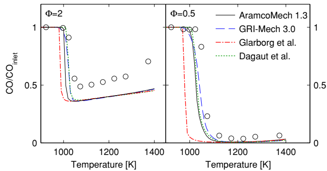
Figure 5: Comparison between modeling results (lines) and data (symbols) from the atmospheric \text{CO}/\text{O}_2/\text{CO}_2/\text{H}_2\text{O}/\text{N}_2 flow reactor of Abián et al. [27]. Inlet conditions: X_{\text{CO}} \approx 5100 ppm, X_{\text{CO}_2} = 25\% , X_{\text{H}_2\text{O}} = 10\% , balance \text{N}_2 .
