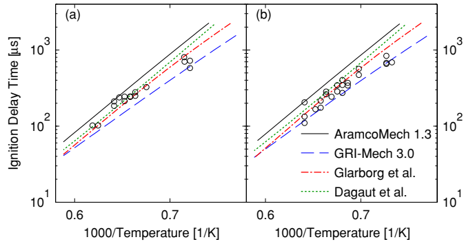
Figure 3: The modeling results (lines) agree well with the experimental data (symbols) of Levy et al. [26] on the ignition delay time of \text{CH}_4 at p = 7\text{-}9 bar, \Phi = 0.3 . (a) \text{N}_2 dilution with 5.2% \text{CO}_2 , (b) \text{N}_2 dilution with 5.2% \text{CO}_2 and 4.0% \text{H}_2\text{O} .
