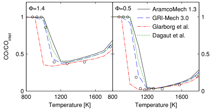
Figure 4: Comparison between modeling results (lines) and data (symbols) from the atmospheric \text{CO}/\text{O}_2/\text{CO}_2/\text{H}_2\text{O}/\text{N}_2 flow reactor of Abián et al. [27]. The modeling was done assuming plug flow with a flow rate of 1 \text{ l}_{\text{STP}}/\text{min} and the temperature profiles given in [63]. Inlet conditions: X_{\text{CO}} \approx 2000 ppm, X_{\text{H}_2\text{O}} = 0.6\% , X_{\text{CO}_2} = 75\% , balance \text{N}_2 .
