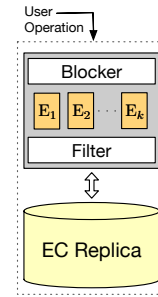
Fig. 3: SYNCOPE
