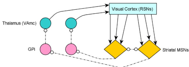
Figure 1: This model is of the closed corticostriatal loop as depicted above. In this figure, dashed lines are inhibitory connections and solid lines are excitatory.
