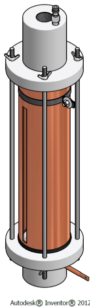
Figure 1. Proposed prototype reactor for water purification (Barillas L)
