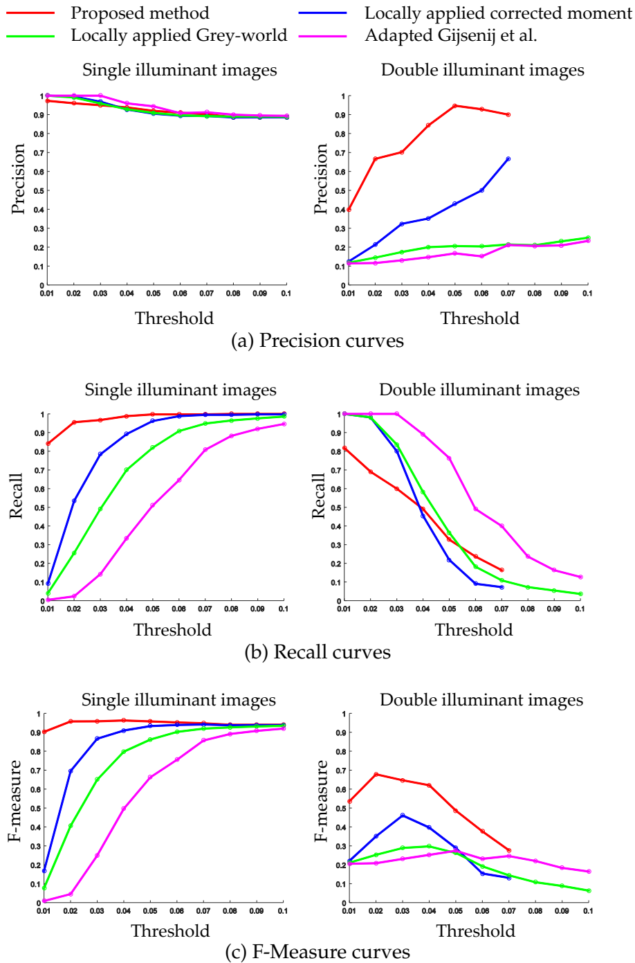
Figure 3.6: Precision, Recall, and F-Measure curves for single and double illuminant images for the four different methods evaluated with the same set of threshold parameter values.
