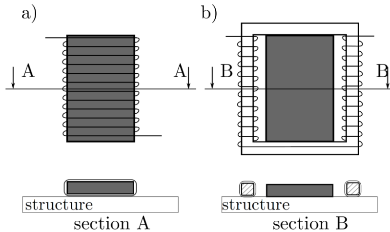
Figure 4. Layouts of traditional configuration (a) and innovative solution (b).
