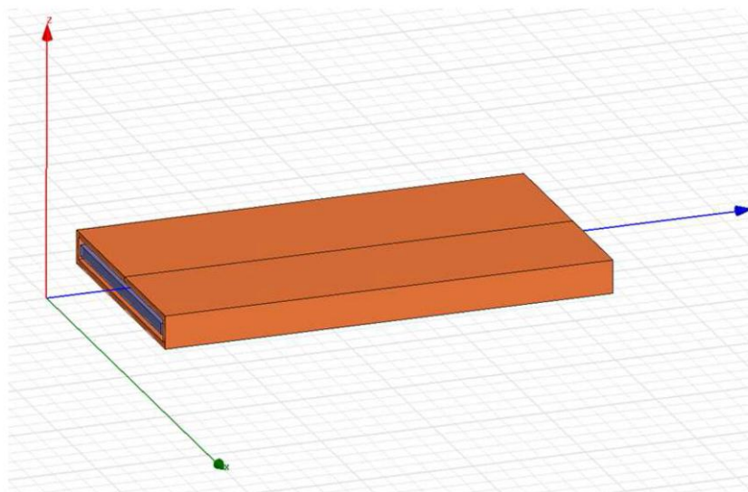
Figure 6. Magnetostrictive patch actuator: traditional layout.
