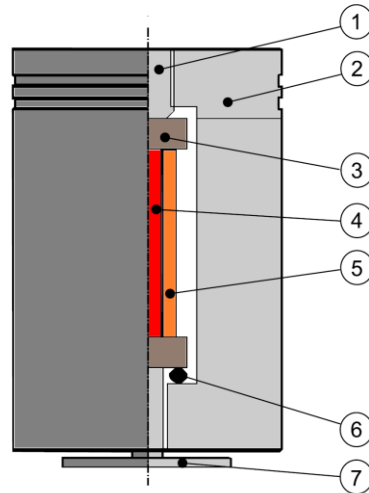
Figure 1. Section of a linear inertial magnetostrictive actuator: (1)-Prestressing screw (2)-Inertial mass, (3)-Permanent Magnets, (4)-Magnetostrictive rod, (5)-Coil, (6)-Spring, (7)-End Effector.
