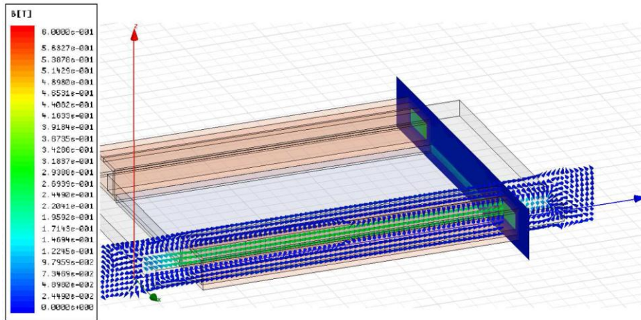
Figure 9. Magnetic field density inside the material: longitudinal section.
