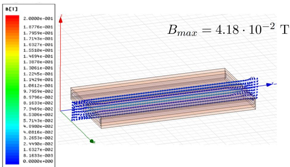
Figure 7. Magnetic field density inside the material.
