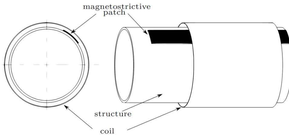
Figure 2. A solution of traditional magnetostrictive patch devices [17].
