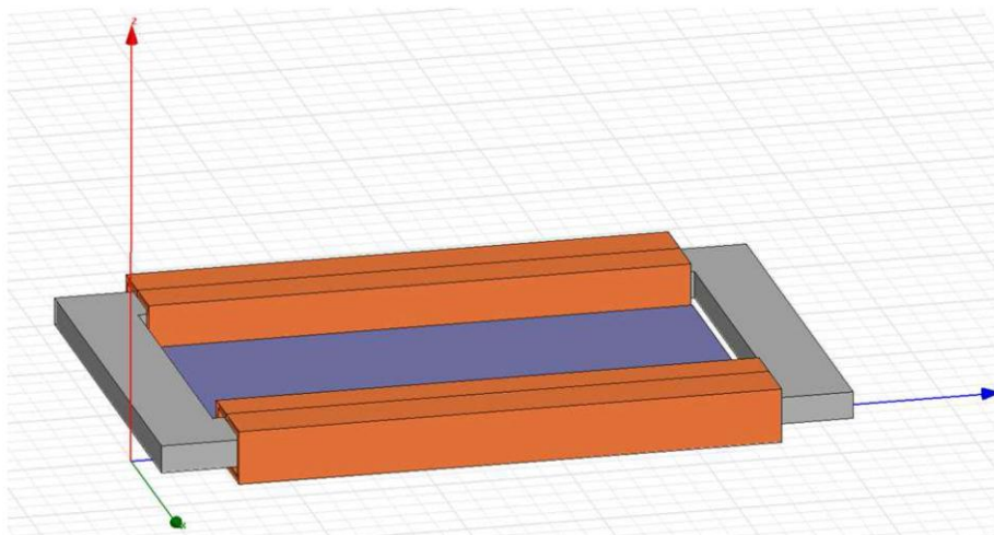
Figure 8. Magnetostrictive patch actuator: innovative layout.
