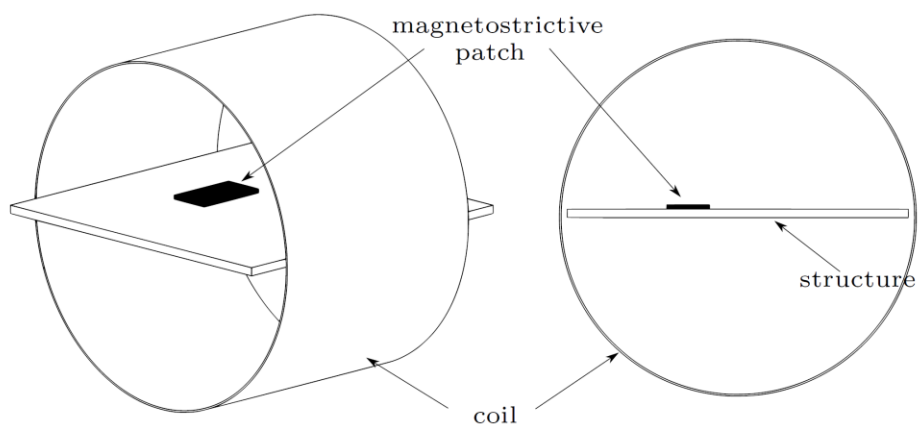
Figure 2. A solution of traditional magnetostrictive patch devices [17].
