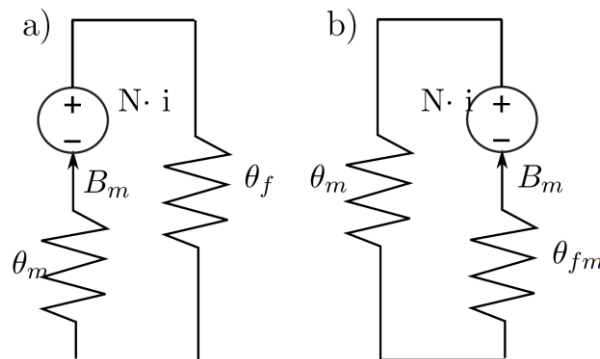
Figure 5. Equivalent magnetic circuits for traditional (a) and innovative (b) layouts.
