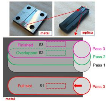
Fig. 1: Micromilled AISI 440 H and its replica.
