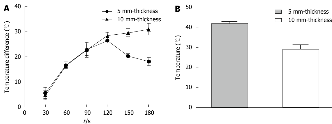
Figure 3 Ex vivo microwave ablation and temperature testing. A: Temperature differences between R1 and R2 when 5 mm-thick and 10 mm-thick gels were maintained; B: Temperatures of R2 when the temperature at R1 was 60 °C. The mean temperature at R2 was 41.9 ± 1.1 °C with a 5 mm-thick gel. When the gel was prepared for 10 mm-thick separation, the mean temperature at R2 was 29.1 ± 2.4 °C.
