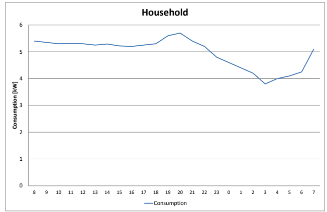
Fig. 5. Solution with optimized tariff: consumption of households CG over time.
