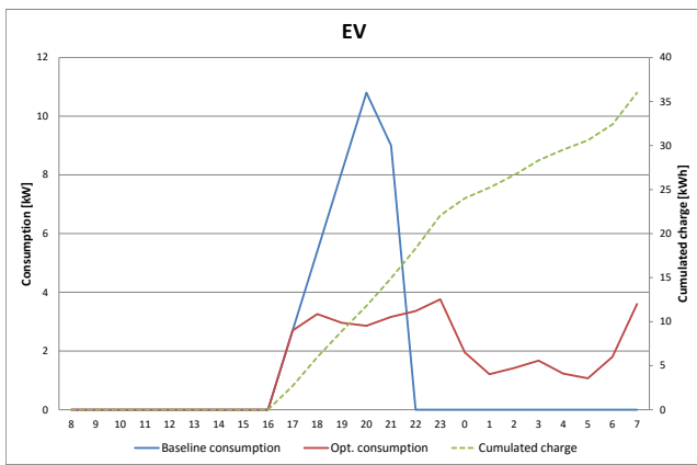
Fig. 4. Solution with optimized tariff: consumption and cumulated load of the electronic vehicle CG over time.
