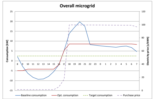
Fig. 2. Solution with optimized tariff: grid-level consumption over time.
