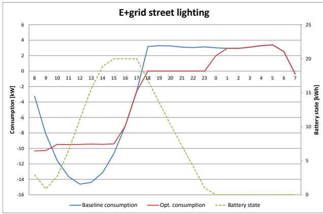
Fig. 3. Solution with optimized tariff: consumption and battery state of the E+grid lighting system CG over time.
