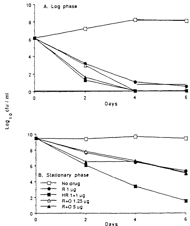
FIG. 3. Bactericidal activities against log-phase (A) and stationary-phase (B) cultures of M. tuberculosis of rifampin alone (R 1 µg) and with isoniazid (HR 1+1 µg) or ofloxacin (R+O 1.25 µg and R+O 5 µg) at the indicated drug concentrations.
