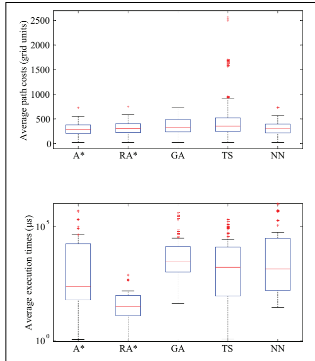
Figure 1. Box plot of the average path costs and the average execution times (log scale) in 100 \times 100 , 500 \times 500 and 1000 \times 1000 random maps of heuristic approaches, tabu search, genetic algorithms and neural network as compared to A^* and RA^* . A^* : A-star; RA^* : relaxed A-star.
