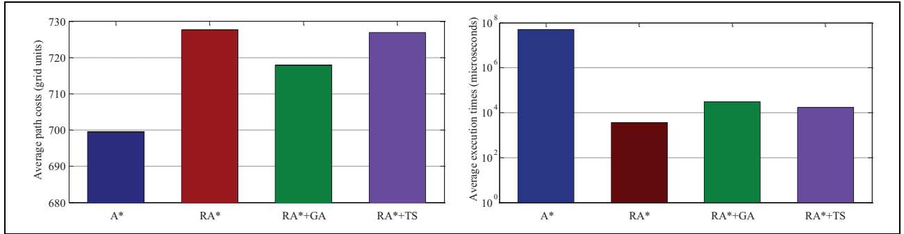
Figure 6. Average path lengths and average execution times (log scale) of hybrid approach RA* + GA and RA* + TS as compared to A* and RA*. RA*: relaxed A-star; A*: A-star; GA: genetic algorithm; TS: tabu search.
