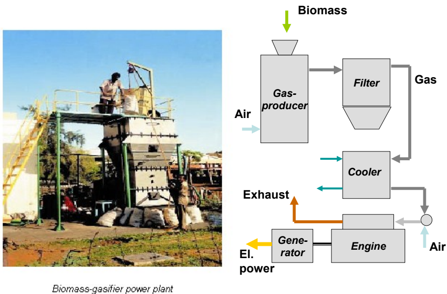
Biomass-gasifier power plant
