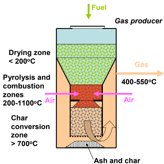
Figure 2. Principle of downdraft gas producer with throat
